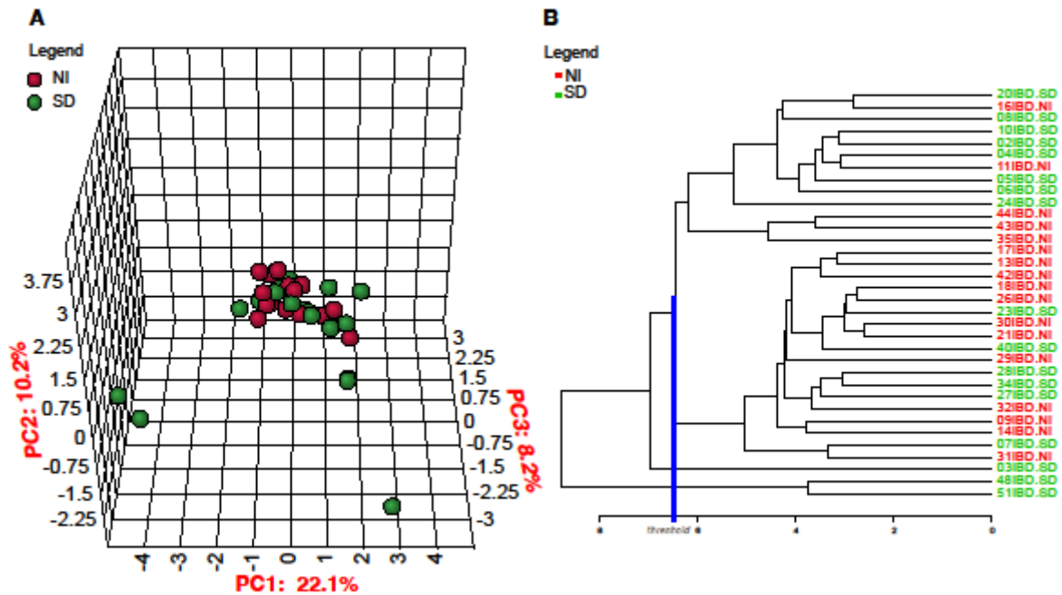
Figure 1. Panel A) Principal component analysis (PCA) from merged metataxonomics and metabolomics results. Taxa and metabolite data were obtained from biological samples (stool and serum, respectively) delivered by IBD volunteers after following the standard diet (SD) or the nutritional intervention (NI) with antioxidants. Panel B) IBD patient clustering based on Euclidean distances. Metataxonomics abundances and metabolomics concentrations from IBD volunteers were both used to obtain the clustering based on the complete algorithm of Euclidean distances.
