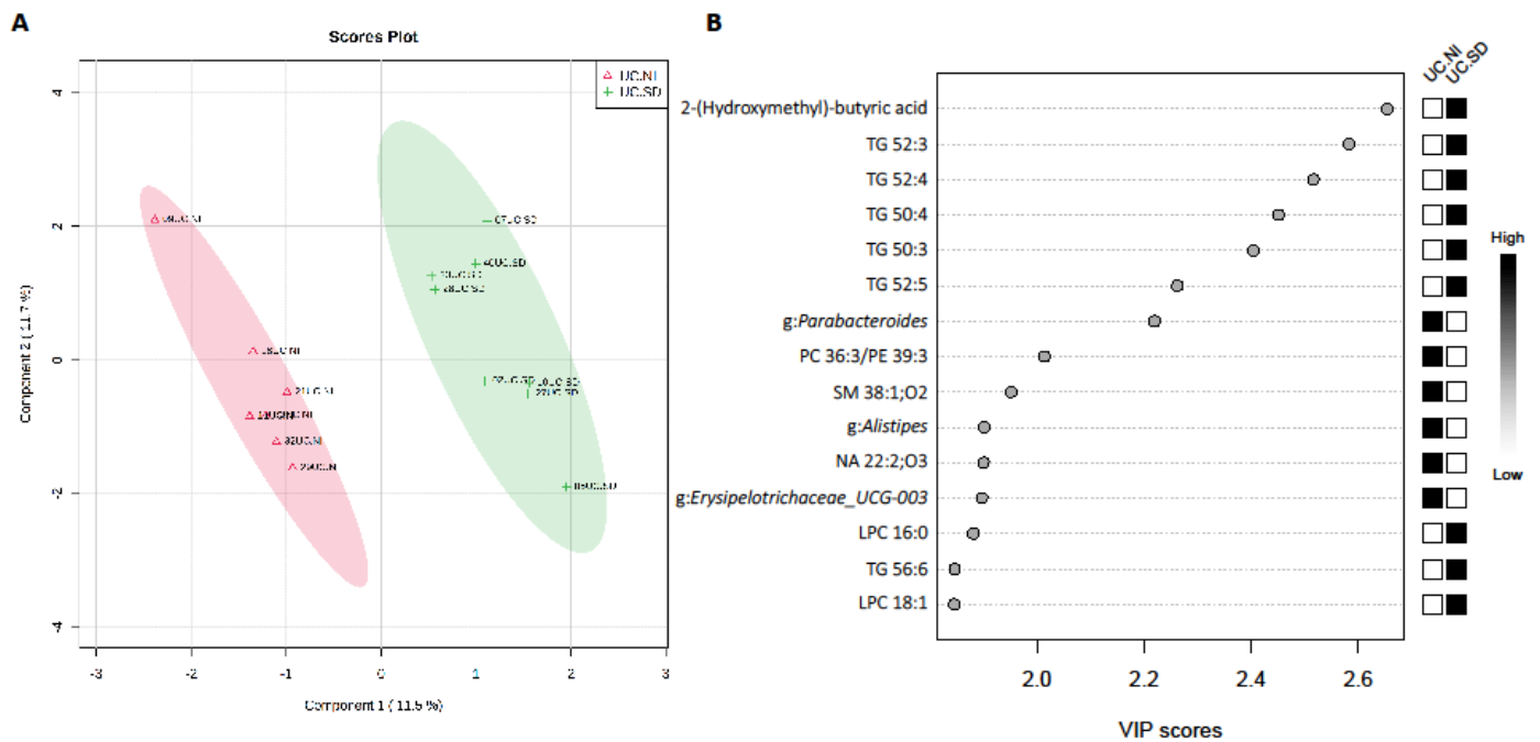
Figure 4. Partial Least-Squares Discriminant Analysis (PLS-DA) in the UC subset. Panel A ) reports the score plot of UC volunteers who delivered samples (feces and blood) after standard diet (SD; green cloud) and nutritional intervention (NI; red cloud) with antioxidants. Clouds were weighted on the 95% of the confidence interval (CI). Panel B ) reports variable important in projection (VIP) scores, ranging from black (high score) to white (low score). Variables included both the concentration of serum metabolites and the relative abundance of the gut taxa.
