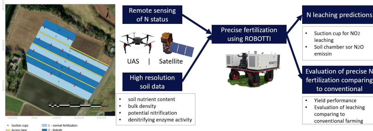
Figure 1. Experimental setup
