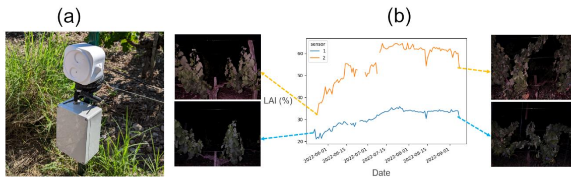
Figure 1. (a) Picture of the sensor in a Château Luchey-Halde vineyard. Bottom case contains the 12V battery powering the system. (b) Example of 2022 LAI time series and images obtained from the monitoring of two grapevines, showcasing different vigor levels.
