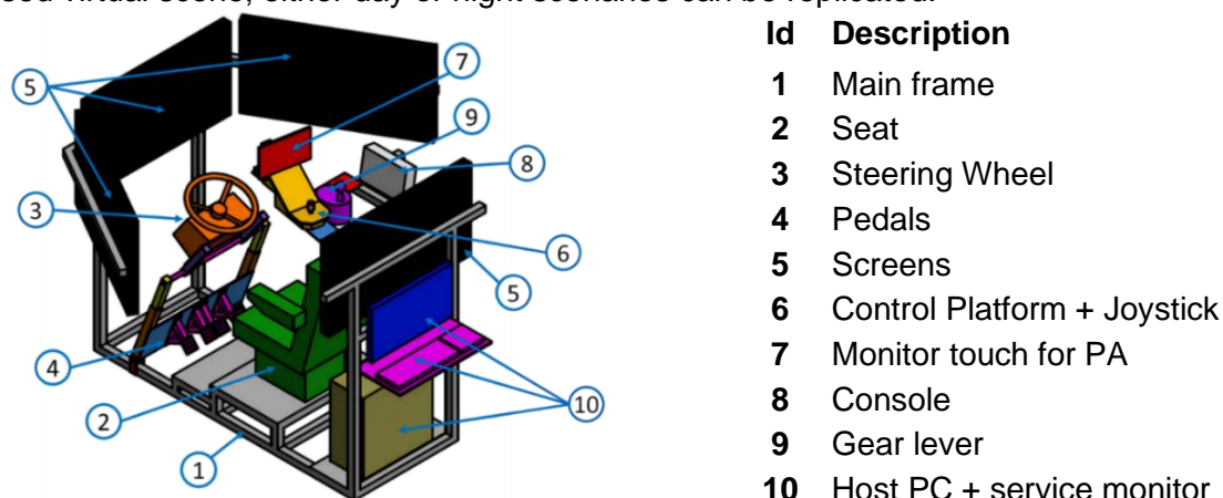
Figure 4 Schema of the static simulator with relevant components.
