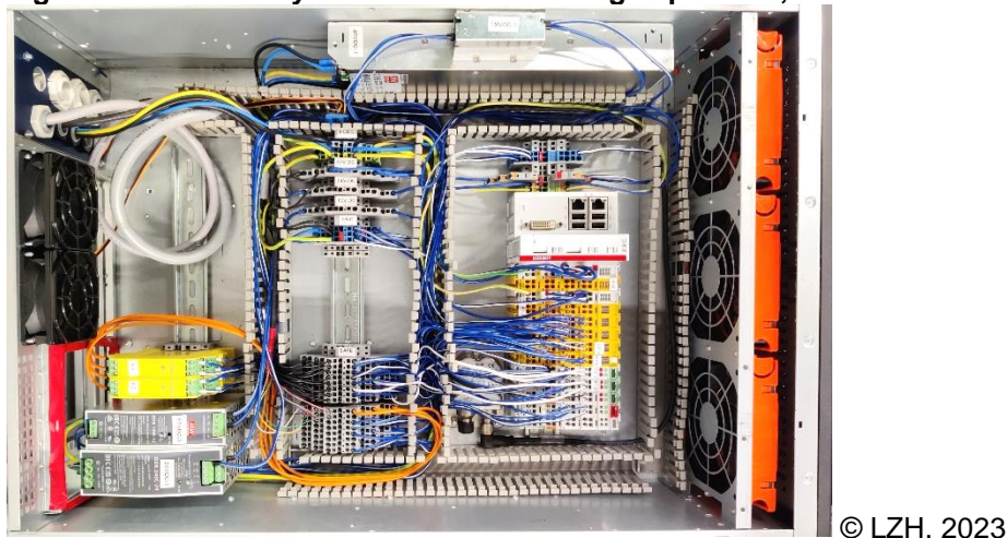
Figure 2. Laser-safety control of the weeding implement, based on a Beckhoff Industrial PC solution.
