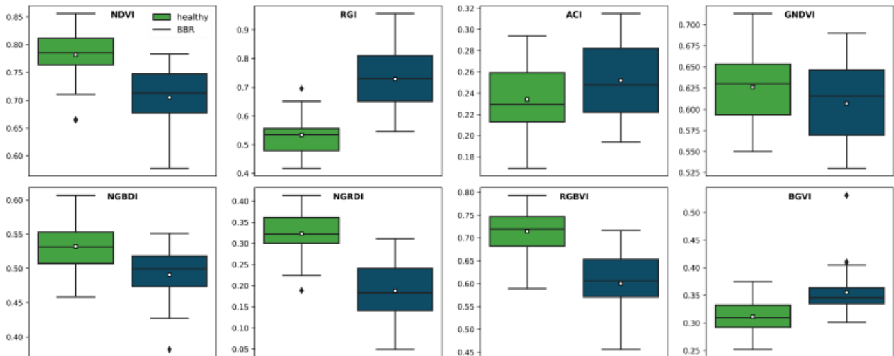
Fig. 2. Boxplots of some of the Vegetation indices.
