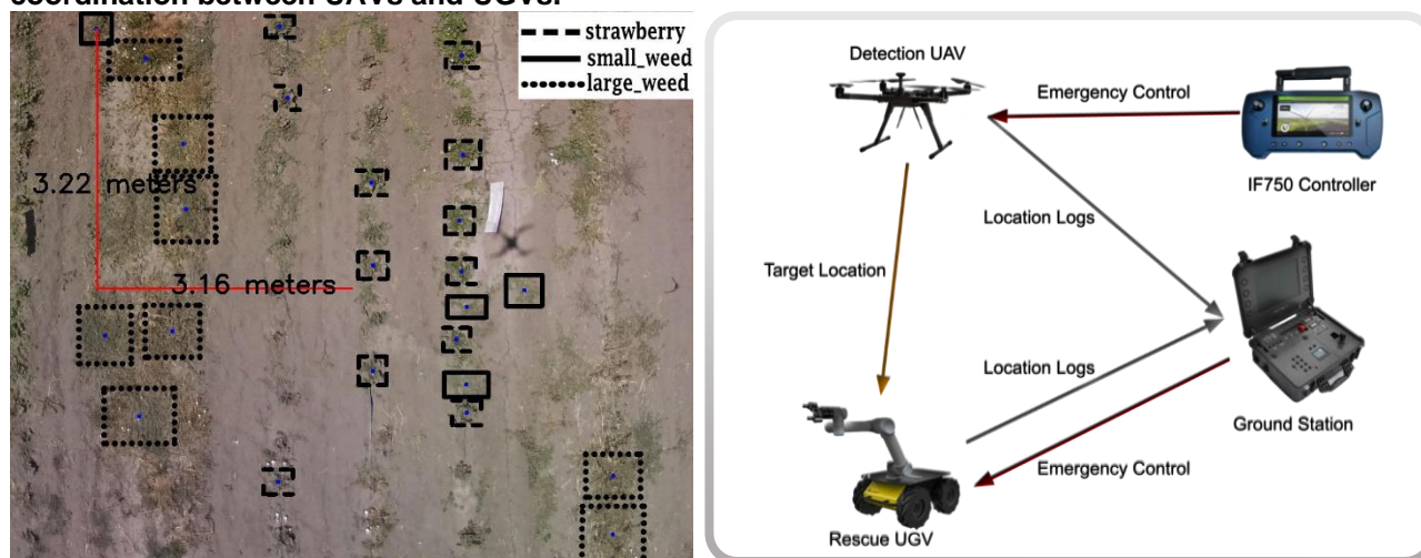
Figure 1. Left: Detected strawberries (dashed bounding boxes), small weeds (solid bounding boxes), and large weeds (dotted bounding boxes). Right: Concept of operation for the autonomous coordination between UAVs and UGVs.
