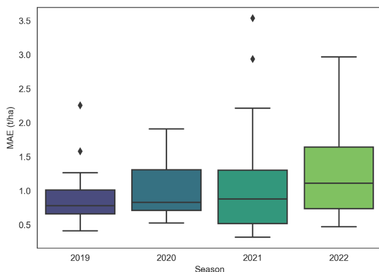
Figure 1. Median, interquartile range and outliers of the mean absolute error (MAE) for the four seasons when estimating the yield of a plot using data from other seasons. The yield of each pixel was estimated, and with the data of all the pixels of each plot, its average error was estimated. The error represented here corresponds to the mean of the errors of the plots used each year.
