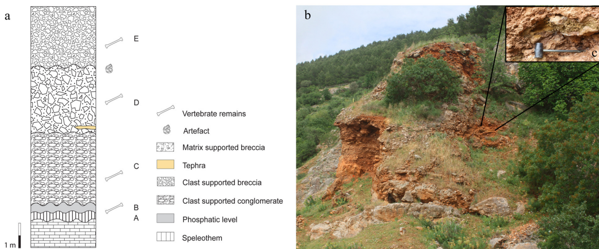
Fig. 2 - Fossiliferous site of Ingarano: a) schematic log of the stratigraphic succession; b) sedimentary succession.
