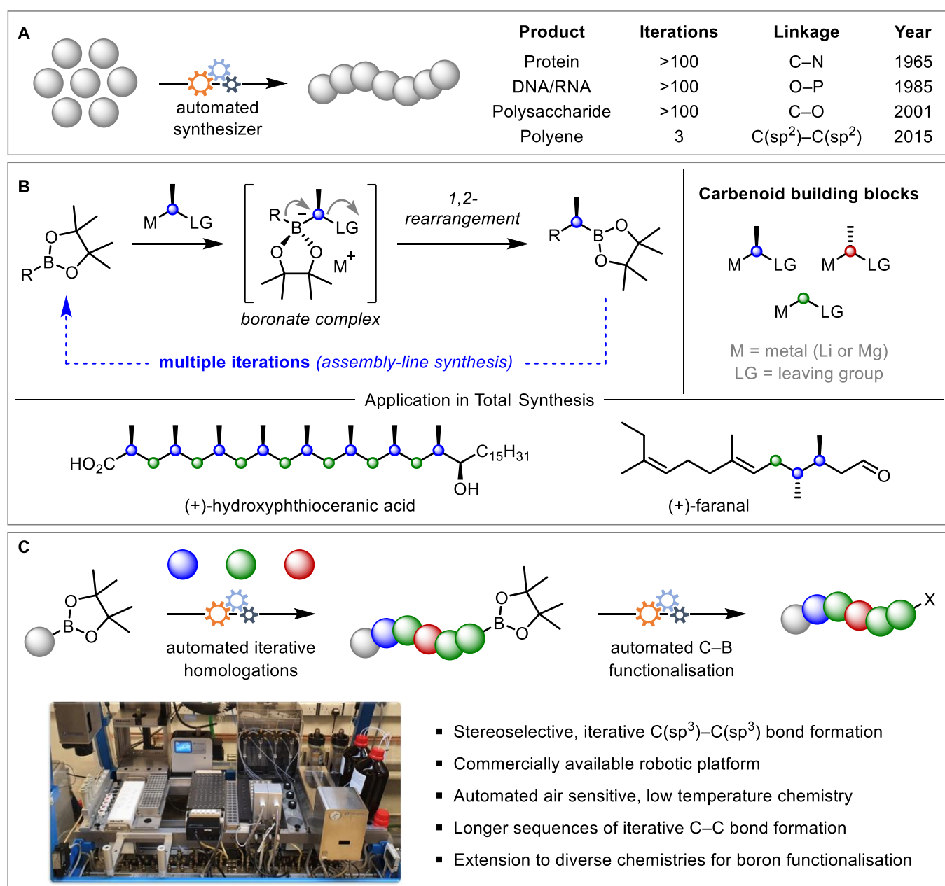
Fig. 1. Automated synthesis development. a, Examples of iterative automated synthesis. b, Assembly-line synthesis by means of homologation of boronic esters and its application in total synthesis. c, Iterative,
