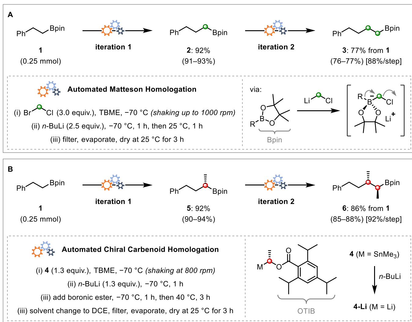
Fig. 2. Automated homologation reactions. a , Automated iterative Matteson homologations. b , Automated iterative chiral carbenoid homologation with lithiated benzoate esters. Yields were determined by 1 H NMR using an internal standard. Yields in parentheses show the range for 4 parallel runs. Bpin = pinacol boronic ester, OTIB = 2,4,6-triisopropylbenzoate.
