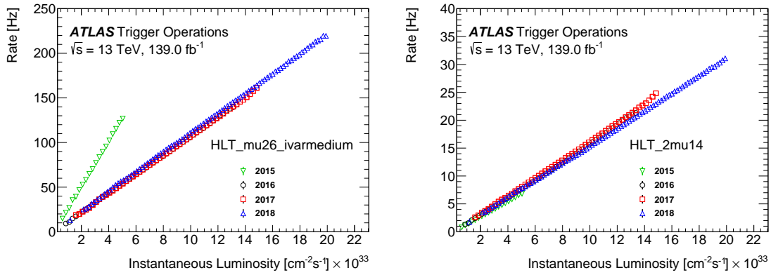
Figure 13. HLT trigger rates as a function of the instantaneous luminosity for the lowest unpre-scaled single-muon and dimuon triggers, HLT_mu26_ivarmedium (left) and HLT_2mu14 (right). The larger rate in 2015 for the single-muon trigger is due to HLT_mu20_iloose_L1MU15 being the lowest unpre-scaled trigger.
