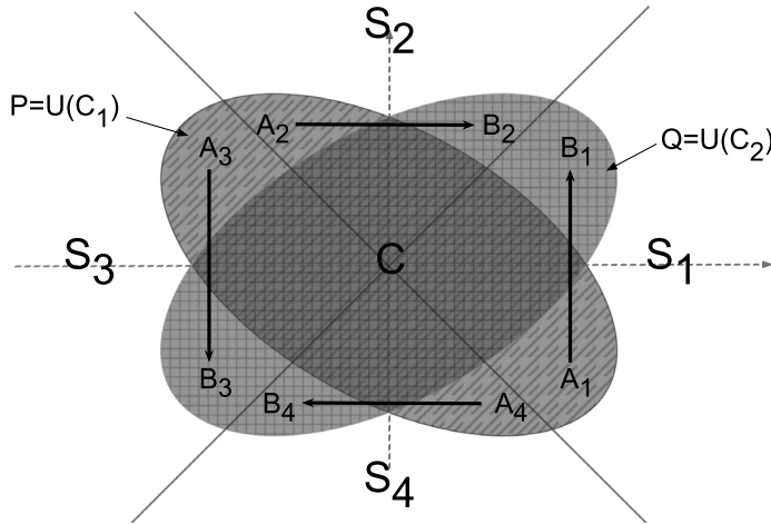
Figure 6. Optimal coupling of two uniform distributions on two rotated ellipsoids. The darker probability mass is not moved.
