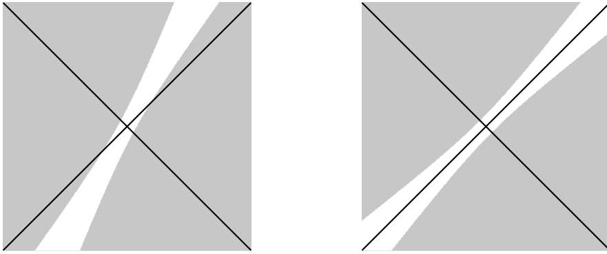
Figure 8. The domains of two reduced Gaussian densities can be rotated (without changing their L^1 -distance) in order to fulfill the symmetry condition (6.3).
