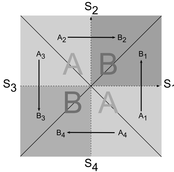
Figure 5. Optimal coupling of two symmetric elliptical distributions with the same generator. The probability mass of the reduced measure P_1 in A_i is reflected onto B_i , for 1 \leq i \leq 4 .
