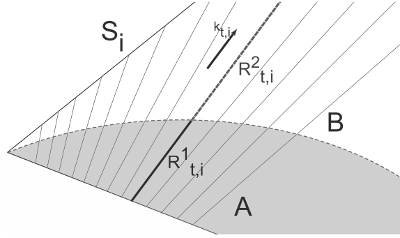
Figure 7. Family of rays R_{t,i} with direction k_{t,i} partitioning the sector S_i .
