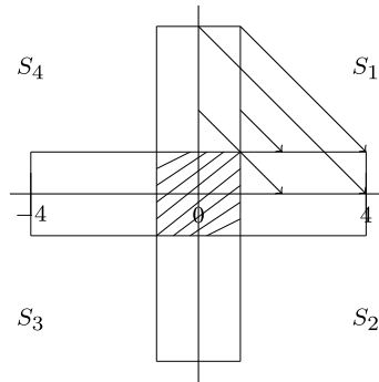
Figure 13. Optimal transport between rotated rectangles
