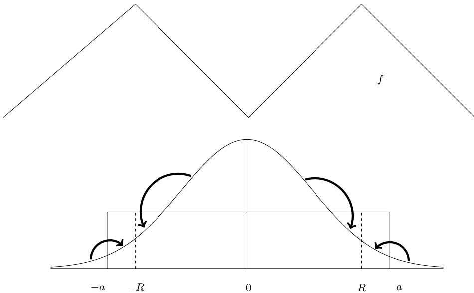
Figure 4. Optimal dual function f and optimal transport between a normal N(0, \sigma^2) and a uniform \mathcal{U}([-a, a]) .
