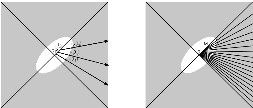
Figure 11. Construction of an approximate optimal coupling on a finite family of rays in the bounded case. Each slice has the same probability with respect to P_1 and Q_1 .
