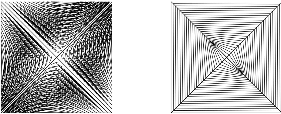
Figure 1. Optimal transportation curves with respect to the squared Euclidean distance ( p = 2 , left) and the Euclidean distance ( p = 1 , right), between the same Gaussian distributions (corresponding to case B in Table 1).
