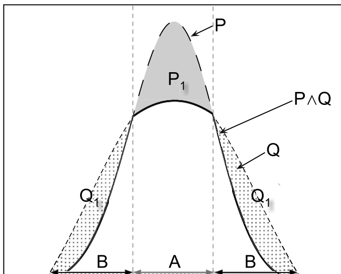
Figure 2. Reduction of measures P, Q to P_1, Q_1 with disjoint supports. To find an optimal transport w.r.t to the l_1 -metric, one does not need to move the white probability mass which is common to P and Q .
