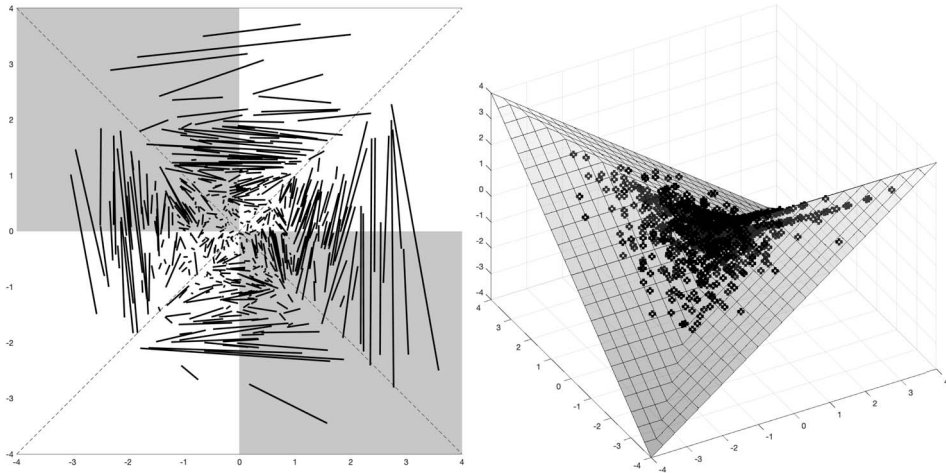
Figure 14. Directions of optimal transport (left) and optimal dual function (right) between discrete versions of the two Gaussian marginals as in case A in Table 1. Discrete Gaussian distributions are obtained via N = 500 simulations. On the left picture we plot the domains of the reduced densities, whereas on the right the exact dual function (7.3) is superimposed on the discretized dual one.
