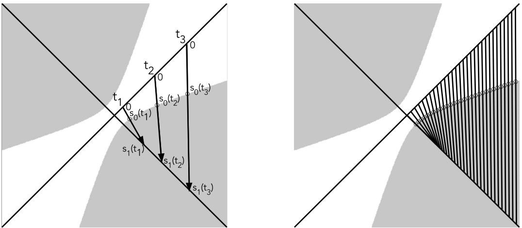
Figure 10. Construction of an approximate optimal coupling on a finite family of rays in the unbounded case. Each slice has the same probability with respect to P_1 and Q_1 .
