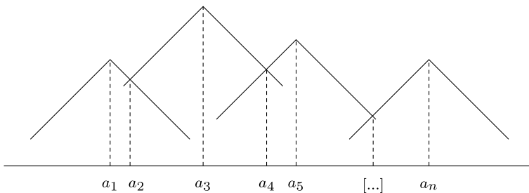
Figure 3. An optimal choice of the dual \ell_1 -convex function f for the \ell_1 -optimal coupling of two distributions intersecting at a finite number of points a_1, \dots, a_n . The gradient of f shows the direction into which mass should be moved.
