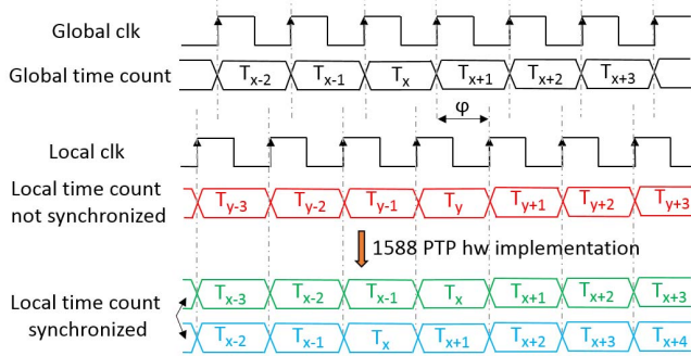
Fig. 3. Temporal diagram of the PTP offset correction mechanism. The theoretical resolution is \pm 1 clock period.
