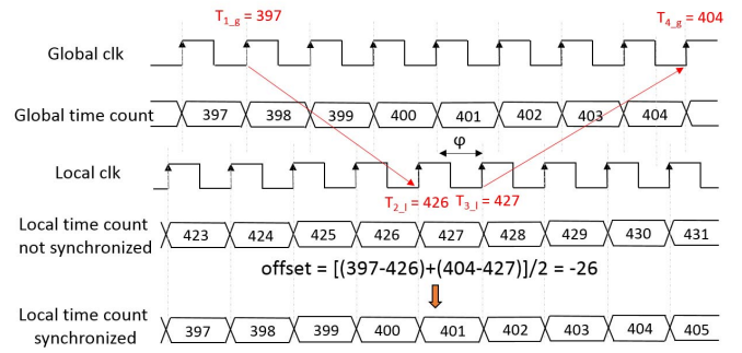
Fig. 5. Numerical example of a negative offset correction.
