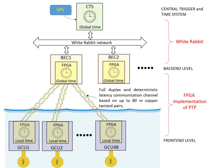
Fig. 1. JUNO readout architecture and synchronization scheme overview.
