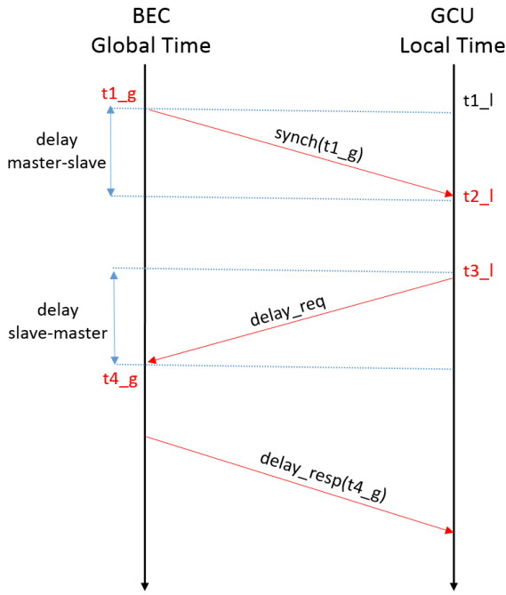
Fig. 2. PTP for offset correction 2008 IEEE.
