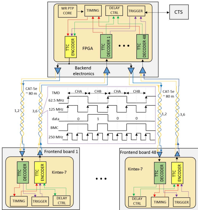
Fig. 7. Multicast messaging physical and data link layers. The implementation of a reliable, full duplex, and fixed latency communication system between master and timing receiver nodes is essential in a message-based synchronization system.
