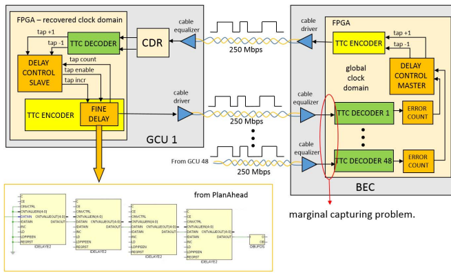
Fig. 9. Serial data streams synchronization overview. The marginal capturing phenomena in the backend electronics has been addressed placing in the front-end logic a cascade of four remotely programmable fine delay primitives.
