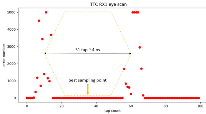
Fig. 11. TTC frame error count versus the tap count yields the information about the eye diagram of the LVDS serial data stream captured in the backend card.
