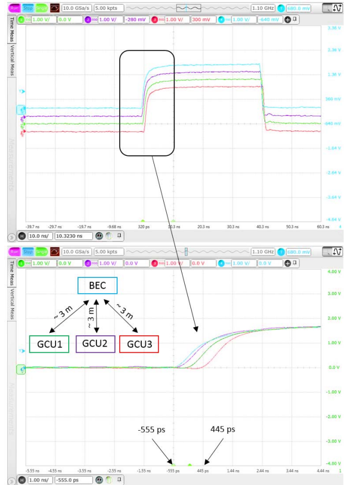
Fig. 12. Timing system test setup composed of one backend and three front-end cards. With 3-m CAT-5e cables, the resolution achieved is about 1 ns.
