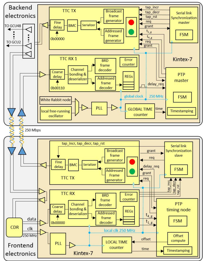
Fig. 8. Complete register transfer level design overview of the IEEE 1588-2008 FPGA implementation.
