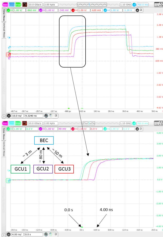
Fig. 13. Time accuracy achieved with a 3-m-long cable channel 1, 80-m-long cable channel 2, and 50-m-long cable channel 3 is slightly larger than 4 ns.
