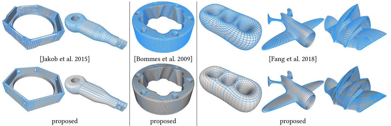
Fig. 25. Because it strives to align close irregular vertices inside patches, our method tends to produce meshes in which the graph of separatrices emanated from irregular vertices (shown in blue) is simpler, compared to competing methods, with fewer edges traversed by separatrices.
