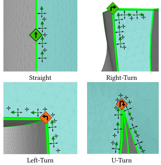
Fig. 6. The four different classes of boundary-vertices of the bluish patch. The classification is defined by the orientation of the green boundary-edges (green arrows) propagated across the cross field (black crosses).
