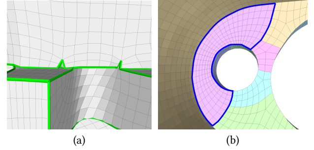
Fig. 22. (a) Miscategorized feature-edges might influence the final quadrangulation; (b) A squeezed patch considered almost perfectly quadrangulable according to the side-length based criteria.
