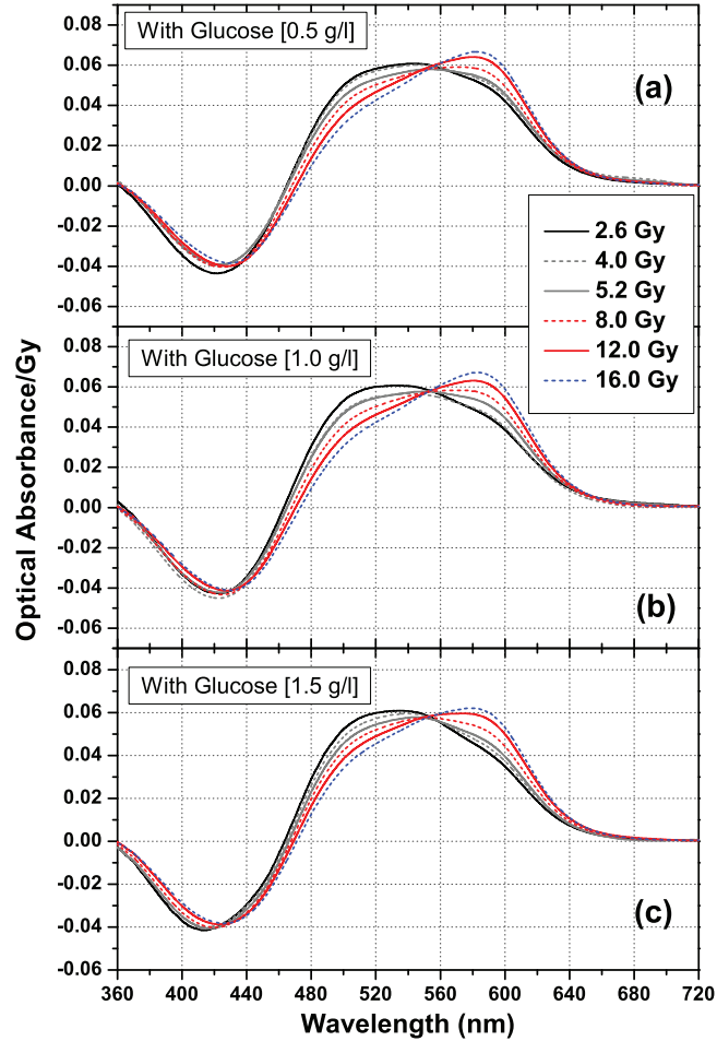
Fig. 8. – Optical absorbance spectra of the various types of gel dosimeters, divided by the absorbed dose. An un-irradiated sample was used as reference. (a) Fricke gel with glucose 0.5 g/l; (b) Fricke gel with glucose 1.0 g/l and (c) Fricke gel with glucose 1.5 g/l.
