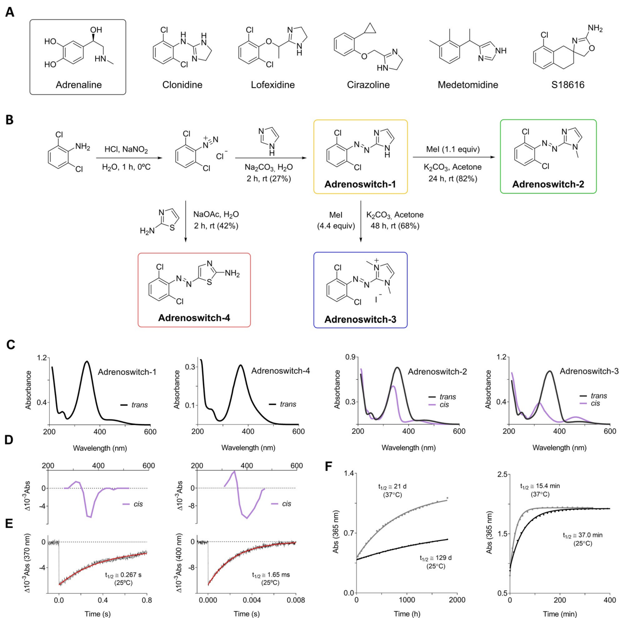
Figure 1. A) Chemical structures of adrenaline and some of the synthetic adrenergic ligands that inspired this work. B) Divergent chemical synthesis of adenoswitches 1–4. C) UV/Vis absorption spectra of the trans isomers. For slow-relaxing adenoswitch-2 and -3, UV/Vis absorption spectra of the cis isomers are also reported. Spectra were extracted from UPLC chromatograms after elution with a mixture of water and acetonitrile supplemented with trifluoroacetic acid. Spectra of cis and trans isomers were normalized at their isosbestic points (see SI—Figures S3A–C). D) Transient absorption spectra of adenoswitch-1 and -4 upon pulsed excitation at \lambda_{\text{exc}} = 355 \text{ nm} in physiological buffer (pH 7.4, 25°C). E) Absorption loss and recovery kinetics of adenoswitch-1 and adenoswitch-4, measured at \lambda = 370 and 400 nm, respectively, upon irradiation with a single ns laser pulse ( t = 0 ) at \lambda_{\text{exc}} = 355 \text{ nm} in physiological buffer (pH 7.4, 25°C). Red lines correspond to monoexponential fitting of the experimental data. F) Cis -to- trans thermal relaxation of adenoswitch-2 and -3 at 25°C (in black) and 37°C (in gray) under dark conditions. Data were fitted to a monoexponential decay model for cis isomers half-lives determination.
