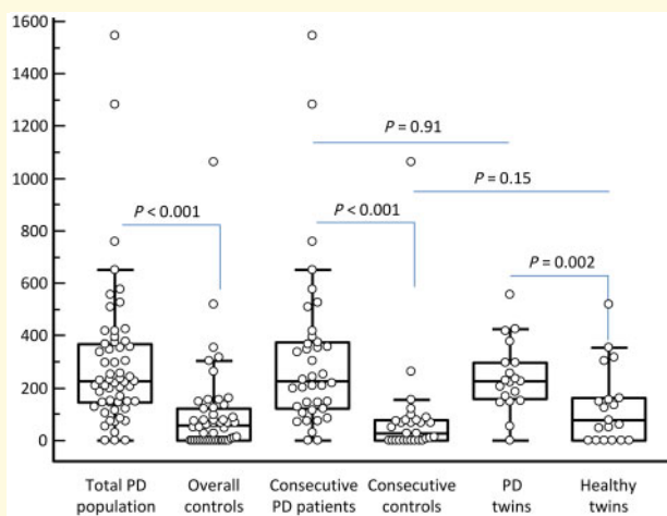
Figure 3 Box and whisker plots of PLA staining in the study population. The box represents the median value (middle line) and the interquartile range (IQR; 25–75th percentile). The external lines extend from the minimum to the maximum value, excluding 'outside' ( \pm 1.5 times the IQR) and 'far out' ( \pm 3 times the IQR) values, which are displayed as separate points. PD = Parkinson's disease.
