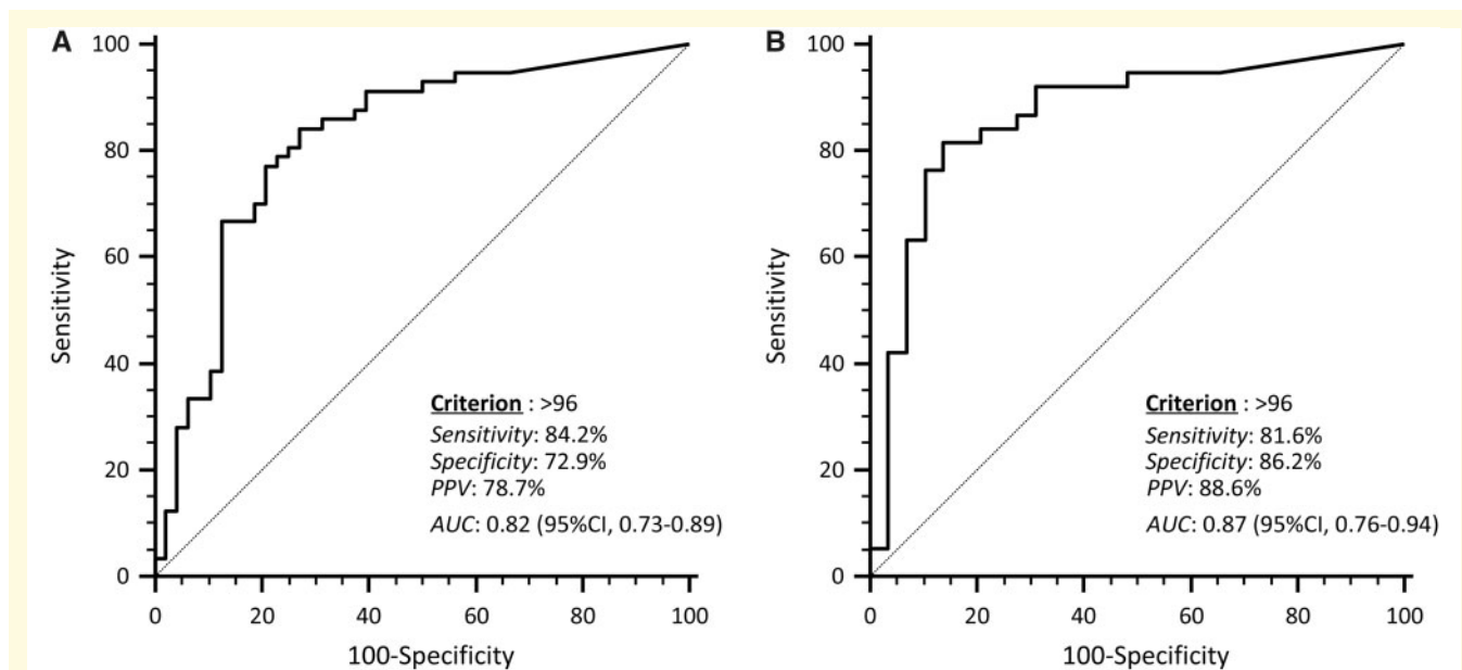
Figure 4 ROC curve analysis of PLA staining score in identifying Parkinson's disease patients. The optimal criterion in the overall population ( A ) and in consecutive Parkinson's disease cases and consecutive healthy controls ( B ) is indicated along with its sensitivity, specificity, positive predictive value (PPV) and the area under the curve (AUC).
