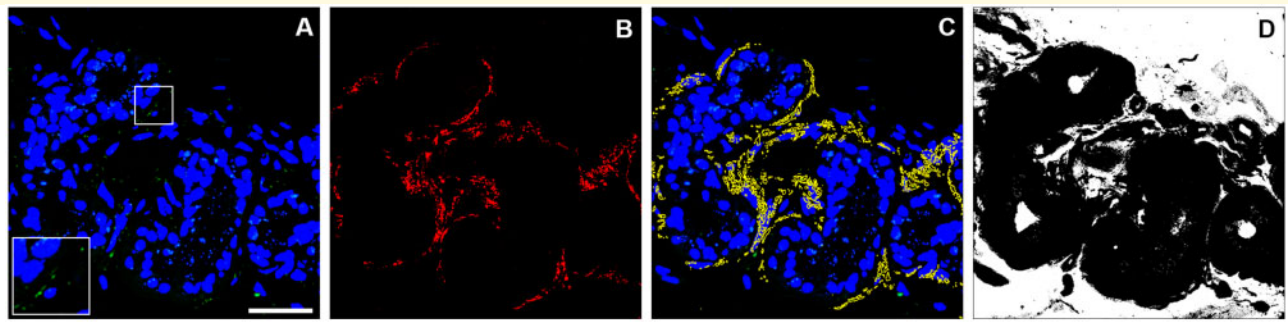
Figure 2 Analytical process in PLA score determination. (A) Representative image of \alpha -synuclein-PLA staining to be quantified. (B) Mask of synaptophysin-positive signal. (C) Superimposition of mask of B (yellow) and A. (D) Total sweat gland area. \alpha -Synuclein-PLA staining (A) was evaluated as the ratio between the area of PLA signal within synaptic terminals and the synaptic density, defined as the ratio between the area of synaptophysin-positive signal (B, red area) and total sweat gland area (D, black area). Inset shows \times 2 magnified view of selected squared area. Scale bar = 20 \mu m. PD = Parkinson's disease.
