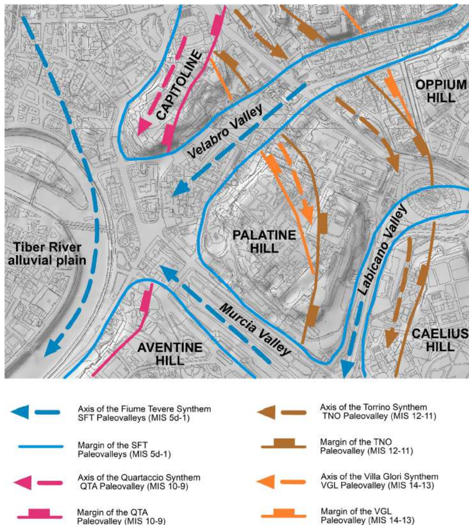
Fig. 10 - Paleogeographic sketch map of the Palatine area showing axes and margins of the main buried paleovalleys (modified and adapted after Alvarez et al., 1996, and Mancini et al., 2014).
