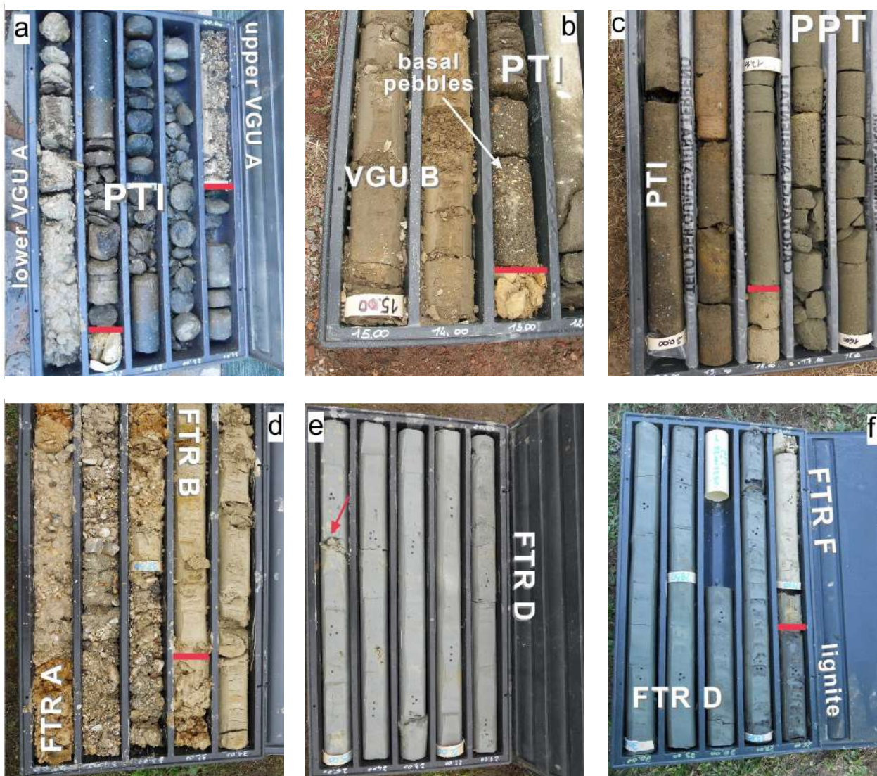
Examples of lithofacies from selected cores (bottoms and tops in the lower left and upper right, respectively; core box is 1 m-long), with main facies boundaries marked in red. a) The Palatino Unit (PTI) ignimbrite interbedded to the fluvial channel gravels of the Valle Giulia Formation (VGU A) from borehole 11 MS (depth interval 25-20 m). b) Very fine-to-fine limestone well-rounded pebbles embedded within the lowermost part of the Palatino Unit (PTI) and the overlying ripple-drift laminated levee sand (VGU B) of the Valle Giulia Formation from borehole 13 MS (depth interval 13-15 m). These pebbles occur mostly in off-valley axis settings and are interpreted to reflect entrainment of fluvial deposits by the PTI pyroclastic flow from the substrate. c) Green-grey, faintly laminated pyroclastic deposit of the Prima Porta Unit (PPT; Middle Pleistocene), overlaying the dark-grey PTI ignimbrite in borehole 16 MS (depth interval 20-15 m). Fosso del Torino Formation (Middle Pleistocene): d) channel gravel (FTR A) with heterometric pebbles in an abundant sandy matrix overlain by cross-laminated fluvial sand of FTR B lithofacies from borehole 22 P (depth 35-30 m); e) pale grey, structureless, silty clay with sparse carbonate nodule (red arrow) interpretable as poorly drained floodplain deposit (FTR D) from borehole 22 P (depth interval 25-20 m); f) blue-grey, structureless, organic-rich clay with a lignite seam on the top interpretable as the deposit of poorly drained floodplain (FTR D) followed upward by yellowish clayey deposits of a well-drained floodplain (FTR F) in borehole 9 MS (depth interval 30-25 m).
