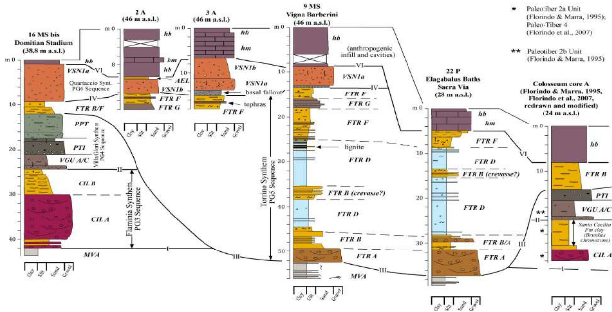
Fig. 9 - Correlated sedimentary logs from selected boreholes in the eastern Palatine Hill and Oppius Hill (see Fig. 2b). Note the internal facies variability of the Fosso del Torrino Formation (FTR) reflecting intercalation of crevasse sandy deposits within floodplain muds. Legend as in Fig. 7.
