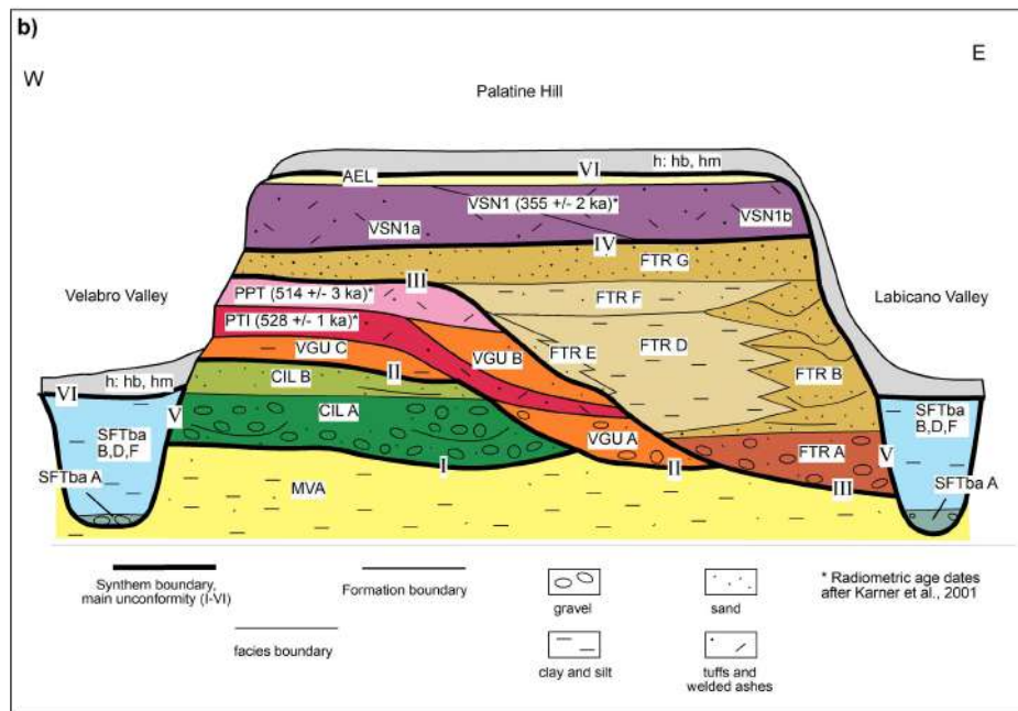
Fig. 3 - a) Chronostratigraphic reference scheme for the Palatine Hill and surrounding areas reporting correlation between (1) sequence stratigraphic units (Milli, 1997), (2) lithostratigraphic and unconformity bounded stratigraphic units (Funicicello & Giordano, 2008) and (3) marine isotope stages (MIS; after Shackleton et al., 1990). b) Simplified sketch of the stratigraphic and facies architecture of the Palatine Hill and the surrounding Labicano and Velabro Valleys (see a in this figure and text for lithostratigraphic and facies codes). In both figures, stratigraphic surfaces I to V are the unconformities bounding the synthem of Funicicello & Giordano (2008), and surface VI is at the base of the man-made deposits.
