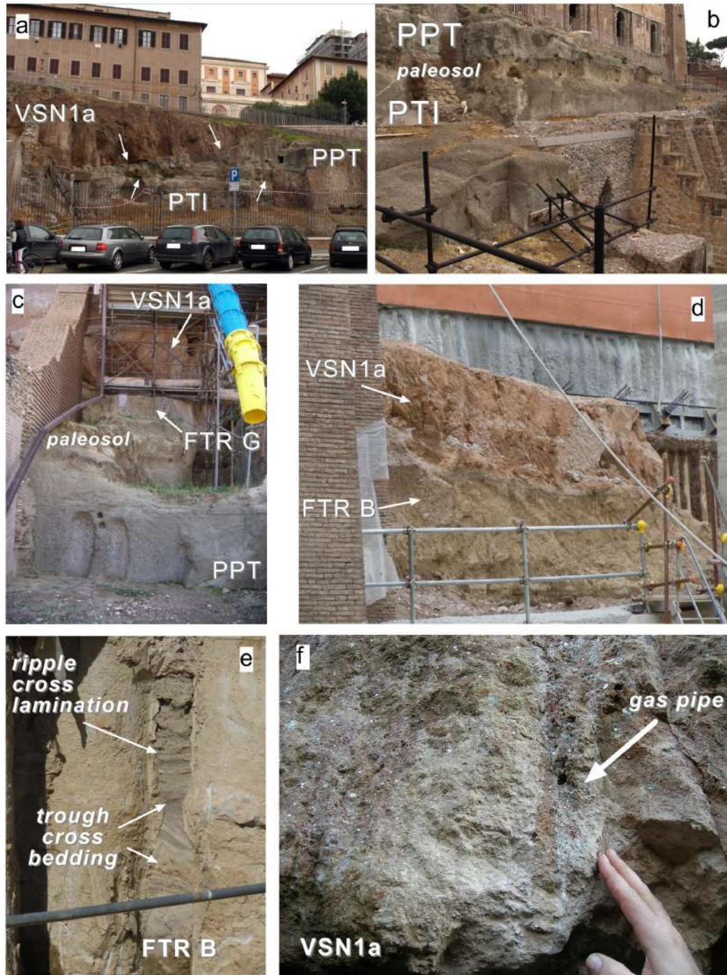
Fig. 6 - a) The superimposed Palatino Unit (PTI), Prima Porta Unit (PPT) and Villa Senni Formation - Tufo Lionato (VSN1a) pyroclastic deposits in outcrop B (Via della Consolazione). b) Detail of outcrop B showing the paleosol separating the Palatino Unit (PTI) from the Prima Porta Unit (PPT). c) Epiclastite of the Fosso del Torrino Formation (FTR G) located between the pyroclastic deposits of the Prima Porta Unit (PPT) below and the Villa Senni Formation - Tufo Lionato (VSN1a) above in outcrop 2 (San Teodoro Church). Note the faintly laminated ashy character as well as the pedogenized top of PPT. d) Detail of outcrop 3, temporarily exposed in April 2015 during the Underground Line C excavations, showing the fluvial channel sand (FTR B) of the Fosso del Torrino Formation, topped by the Villa Senni Formation - Tufo Lionato (VSN1a) ignimbrites. e) Detail of outcrop 4, temporarily exposed in May 2018 during the Underground Line C excavations, showing trough-cross bedded and cross laminated sands (FTR B) of the fluvial Fosso del Torrino Formation. Outcrops 3 and 4 are remnants of the former Velia Hill, cut away in the 30s of the XX century for the construction of Via dei Fori Imperiali (De Angelis D'Ossat, 1956; Lanzini, 2008; Leone et al., 2009). f) Detail of outcrop 2 showing a columnar gas pipe from the Tufo Lionato ignimbrite (VSN1a).
