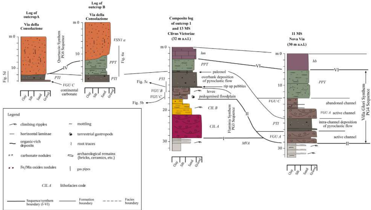
Fig. 7 - Correlated sedimentary logs from selected boreholes and key outcrops along the Velabro Valley and in the north-western Palatine (see Fig. 2b for location).
