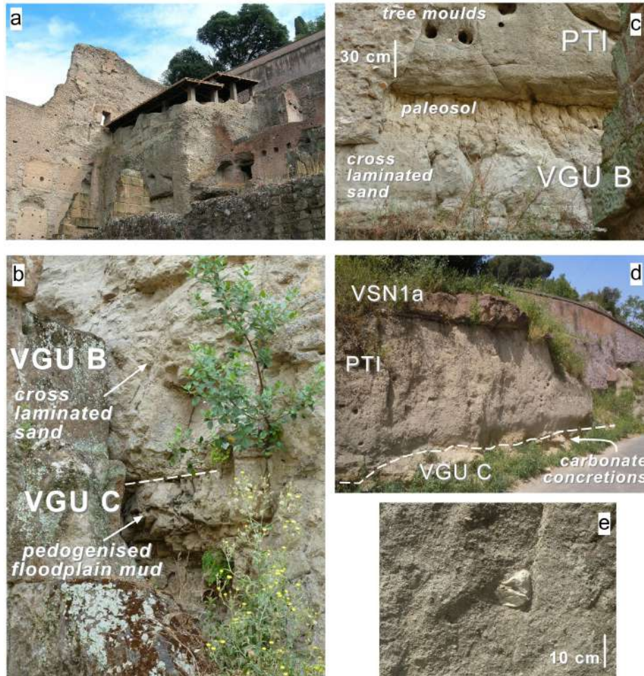
Fig. 5 - Pictures of key outcrops discussed in the text (see Fig. 2b for reference and location). a) Roman walls and foundation structures along the north-western side of the Palatine. Note how these ruins sit directly on top of outcrop 1 (see details in this figure). b) Detail of the lowermost part of outcrop 1 showing pedogenized floodplain mud (VGU C) capped by cross-laminated levee sand (VGU B) from the fluvial Valle Giulia Formation. c) Detail of outcrop 1 showing cross-laminated levee deposits with a well-developed paleosol on top (VGU B lithofacies) overlain with a sharp but non-erosive contact by the massive ignimbritic Palatino Unit (PTI). Note the presence of tree moulds in PTI, previously described by De Rita et al. (2002). d) From base to top, carbonate-rich silts and concretions (VGU C lithofacies) and the PTI and the Villa Senni Formation (VSN) ignimbrites exposed in outcrop A (Via della Consolazione, southern hillslope of the Capitoline Hill). e) Detail of the PTI ignimbrite in outcrop A showing a sub-angular, carbonate lithic fragment, most likely a xenolith (see e.g. Funicello & Parotto, 1978).
