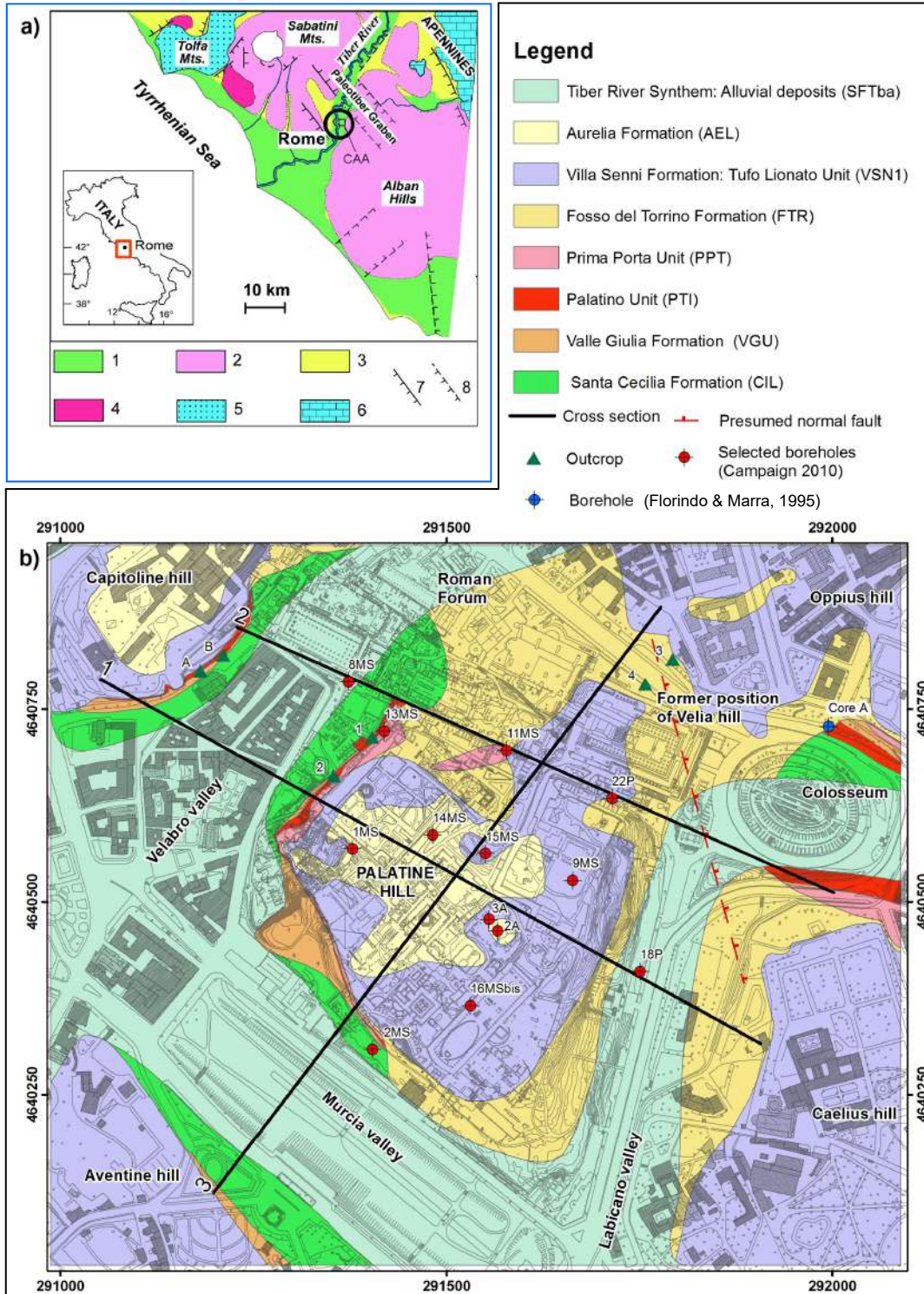
Fig. 2 - a) Simplified geological map of the Rome Basin. Legend: 1) continental and coastal deposits (late Early Pleistocene-Holocene); 2) pyroclastic deposits and lavas of the Sabatini Mts and Alban Hills Volcanic Districts (Middle-Late Pleistocene); 3) marine terrigenous clay and sands (Pliocene-Early Pleistocene); 4) lavas and lava domes of the Ceriti Mts-Tolfa Volcanic District (Pliocene); 5) marine terrigenous successions of the Liguride Units, sandstones and marlstones (Cretaceous-Paleogene); 6) limestone, marls and cherts of the pelagic Umbro-Sabina succession (Trias-Miocene); 7) normal fault; 8) buried normal fault. CAA is the Central Archeological Area of Rome. b) Geological map (modified, after Mancini et al., 2014) showing the distribution of lithostratigraphic units below the anthropogenic deposits with location of cross-sections of Fig. 4, outcrops pictured in Figs. 5 and 6, and borehole stratigraphies detailed in Figs. 7-9.
