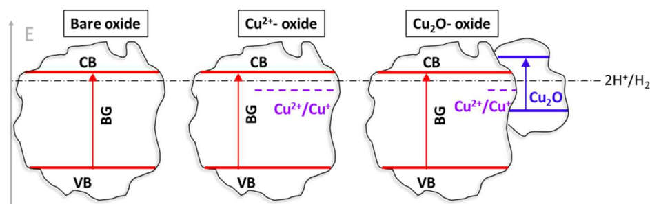
Figure 3. Schematic representation of the band structure alignment of bare and Cu modified samples. The case here reported is that of \text{TiO}_2 (T). In the case of zirconium titanate (ZT) the situation is analogous.
