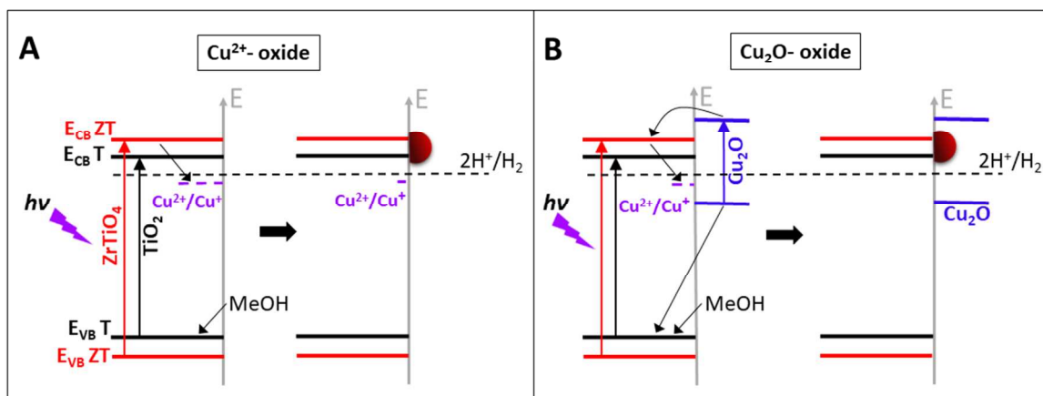
Figure 9. Chemical modifications occurring at the surface of the different Cu modified samples during \text{H}_2 evolution reaction.
