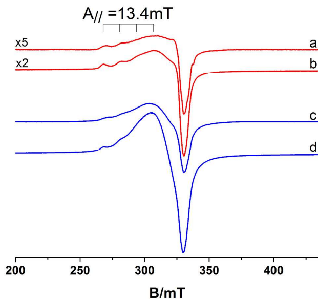
Figure 2. EPR spectra of the Cu modified samples recorded at low temperature under vacuum condition. a) \text{Cu}_2\text{O} -T, b) \text{Cu}_2\text{O} -ZT, c) \text{Cu}^{2+} -T and d) \text{Cu}^{2+} -ZT sample.
