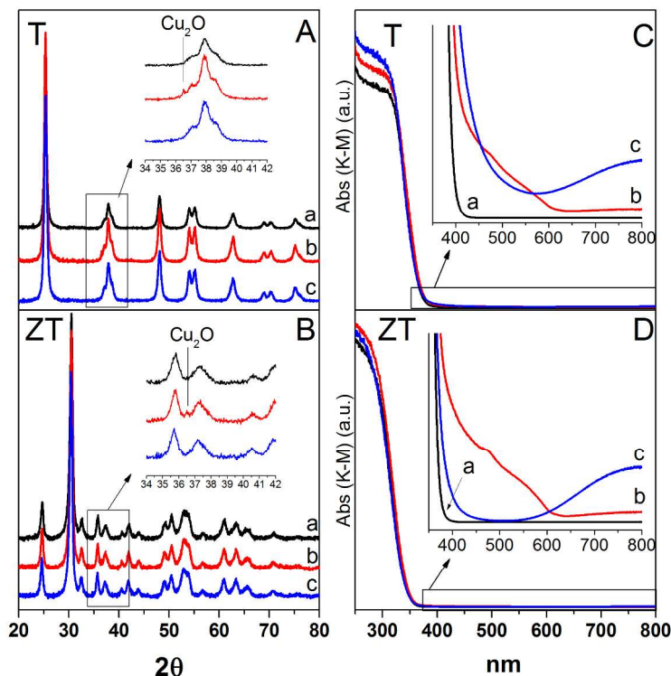
Figure 1. XRD diffractograms (panel A and B) and DR-UV-Vis spectra (panel C and D) of the bare oxides and the corresponding Cu modified materials. Panel A and C. \text{TiO}_2 based materials: a) T, b) \text{Cu}_2\text{O} -T and c) \text{Cu}^{2+} -T. Panel B and D. \text{ZrTiO}_4 based materials: a) ZT, b) \text{Cu}_2\text{O} -ZT and c) \text{Cu}^{2+} -ZT. The diffraction patterns shown in panel A are due to the anatase polymorph of \text{TiO}_2 except for the feature shown in the inset which corresponds to the (111) reflection of cuprite ( \text{Cu}_2\text{O} ). The diffraction patterns shown in panel B correspond to the scrutinyite structure ( \text{ZrTiO}_4 ). Again, the feature highlighted in the inset corresponds to the (111) reflection of cuprite ( \text{Cu}_2\text{O} ).
