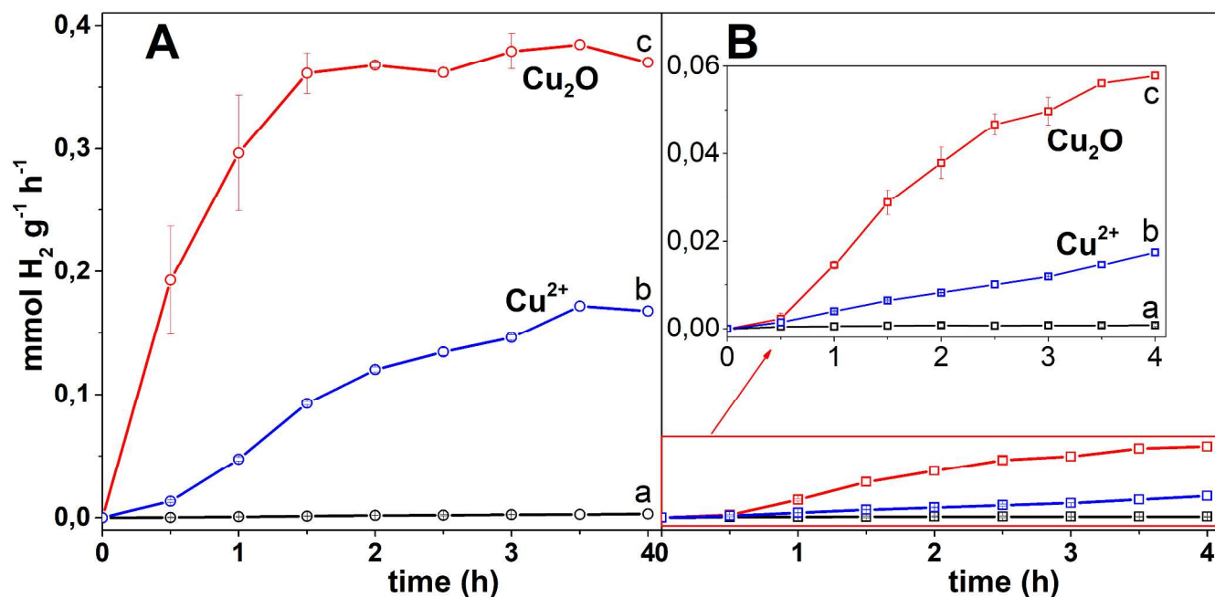
Figure 4. Hydrogen evolution rate ( \text{mmol g}^{-1} \text{h}^{-1} ) obtained with (A) \text{TiO}_2 based samples; (B) \text{ZrTiO}_4 based samples. a) bare oxides, b) \text{Cu}^{2+} -oxides and c) \text{Cu}_2\text{O} -oxides.
