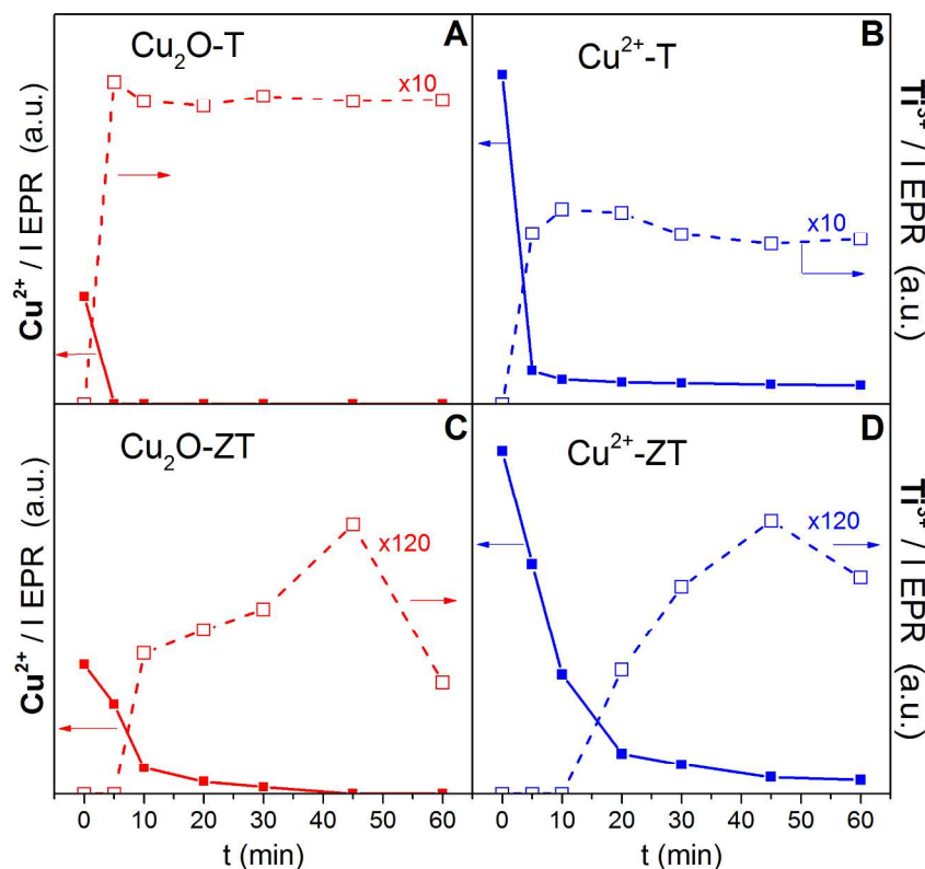
26 27 28 29 30 31 32 33 34 35 36 37 38 39 40 41 42 43 44 45 46 47 48 49 50 51 52 53 54 Figure 7. EPR intensities of \text{Cu}^{2+} (straight lines) and \text{Ti}^{3+} species (dashed lines) at different times of UV-Vis irradiation of 55 \text{Cu}_2\text{O} -oxides (panels A and C, red lines) and \text{Cu}^{2+} -oxides (panels B and D, blue lines) in methanol/water suspension.
