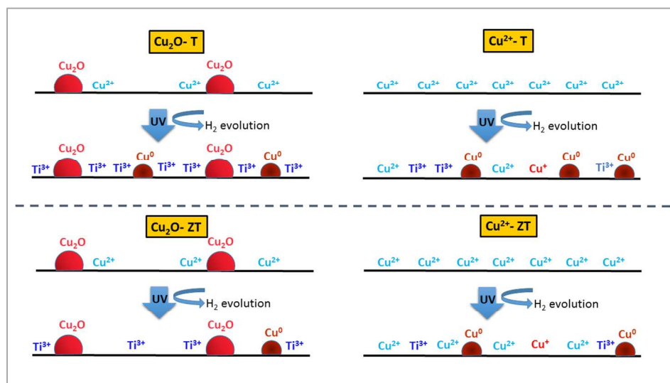
Figure 9. Chemical modifications occurring at the surface of the different Cu modified samples during \text{H}_2 evolution reaction.
