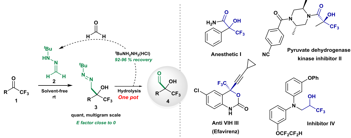
Scheme 1. \alpha -Hydroxy aldehydes 4 as building blocks in target-oriented synthesis.
