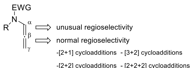
Scheme 1. Regioselectivity patterns in Gold Catalyzed [n+2] cycloadditions.
