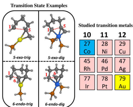
Figure 1 Studied transition metals and example transition states (5- exo - & 6- endo - trig with gold (yellow); 5- exo - & 6- endo - dig with cobalt (blue)).
