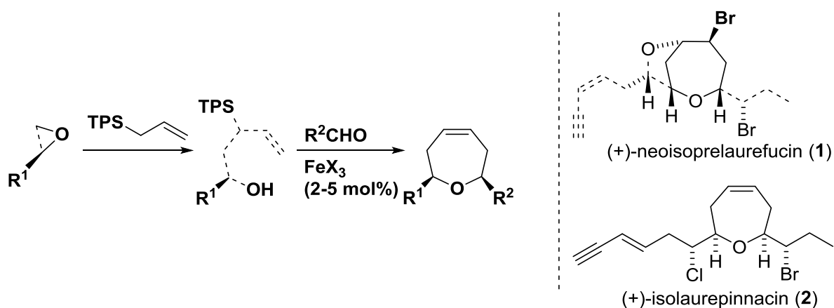
Scheme 1. Synthesis of \Delta^4 2,7-disubstituted oxepenes.
