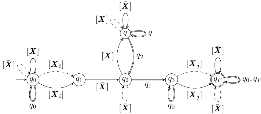
FIG. 11. OPA for atomic formula \psi = X_i \sim X_j .
