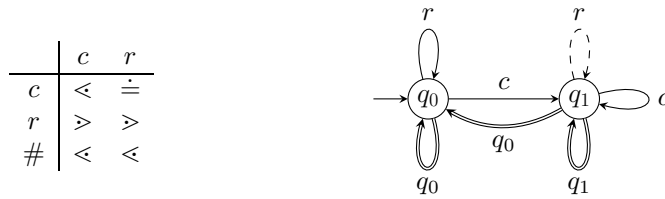
FIG. 16. \omega DOPMA and \omega DOPBEA recognizing L_{\omega\text{Dyck-pr}(c,r)} .
