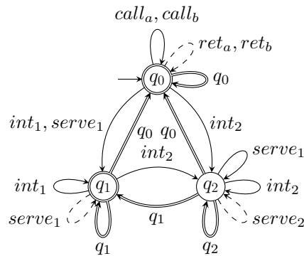
FIG. 13. \omega OPBA recognizing the language of Example 8.
