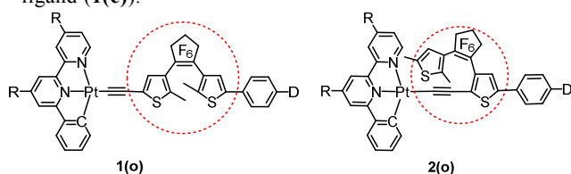
Chart 1 Chemical structures of DTE-based ( N^N^C )Pt(II) complexes 1 , ( R = \text{Hex} , D = \text{NMe}_2 ) and 2 ( R = \text{tBu} , D = \text{NBu}_2 )
