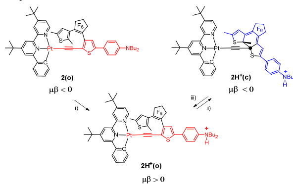
Scheme 1 A three-state system: complex 2(o) and the protonated open-DTE isomer 2H + (o) and closed-ring isomer 2H + (c) . i) \text{HBF}_4 \cdot \text{OEt}_2 , \text{CH}_2\text{Cl}_2 ; ii) \text{CH}_2\text{Cl}_2 , h\nu (350 nm); iii) \text{CH}_2\text{Cl}_2 , h\nu (580 nm).
