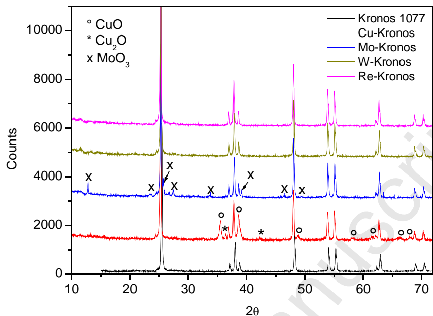
Figure 1: XRD patterns of bare and decorated Kronos 1077
