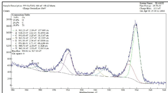
Figure 8 XPS: Cu high-resolution spectrum.
