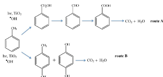
Figure 11: Toluene oxidation reaction pathway [22].
