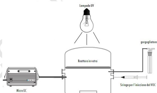
Figure 10: Photoreactor gas-phase system scheme.
