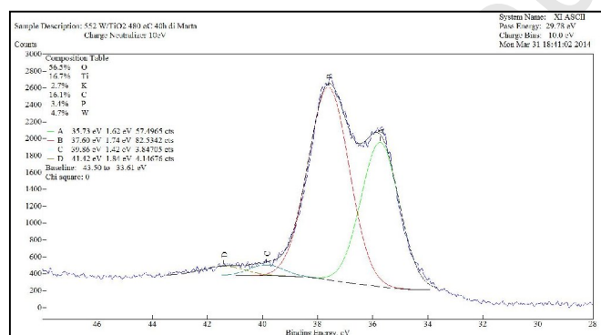
Figure 7 XPS: W high-resolution spectrum.
