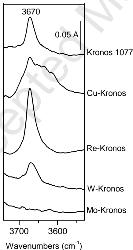
Figure 9: FT-IR spectra.
