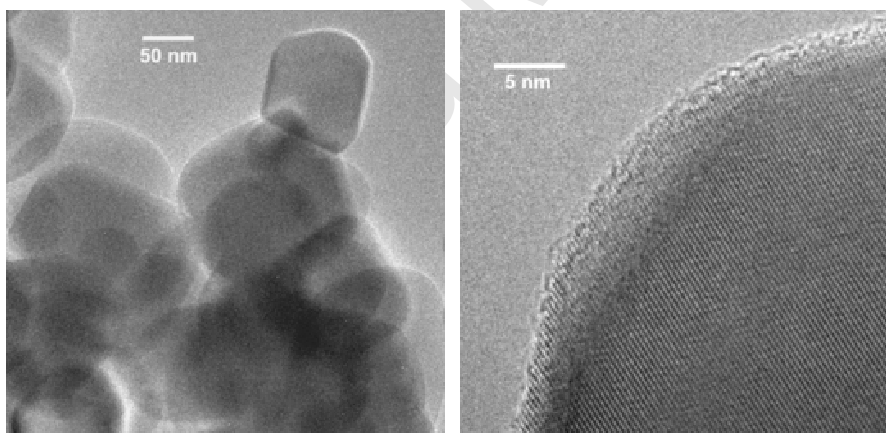
Figure 2: TEM images of Kronos 1077.
