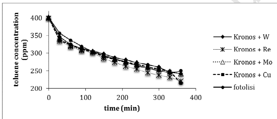
Figure 12: Toluene photodegradation in gas-phase under UV irradiation [Toluene concentration] vs. time
