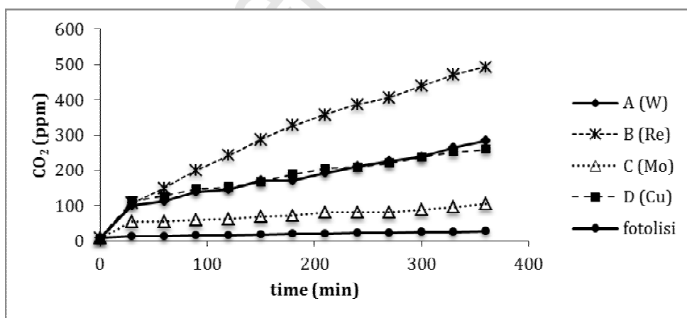
Figure 13: CO 2 formation during the photodegradation process
