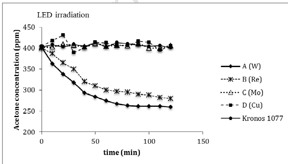
Figure 15: Acetone photodegradation in gas-phase under visible light (performed with a LED lamp).
