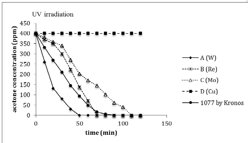
Figure 14: Acetone photodegradation in gas-phase under UV irradiation.
