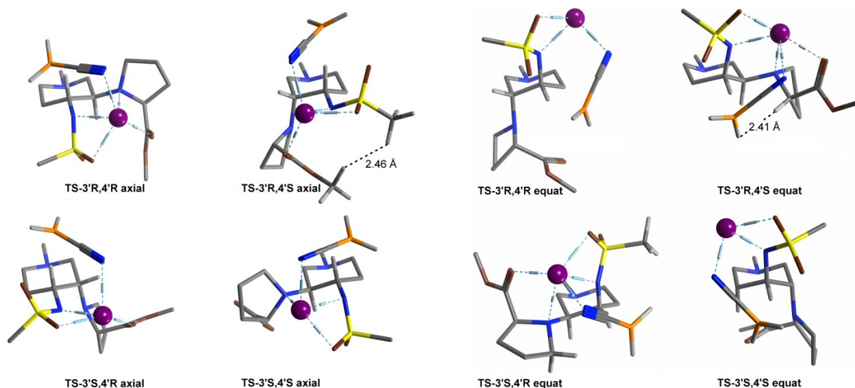
Figure 2. Geometries of all the possible TSs deriving from either the axial or equatorial attack of the hydride.
