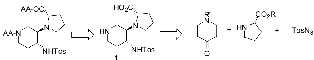
Scheme 1. Retrosynthesis of reverse turn peptidomimetic
