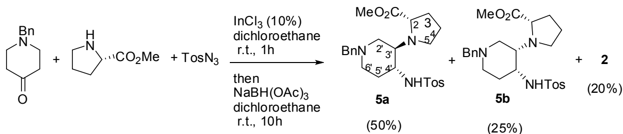
Scheme 3. Scale up of multicomponent reaction
