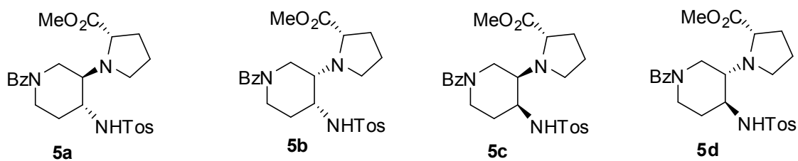
Figure 1. Possible stereoisomers of 5
