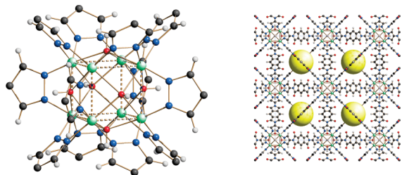
Figure 1. Left: drawing of the \text{Ni}_8(\mu_4\text{-X})_6(\mu_4\text{-L})_6 cluster ( \text{X} = hydroxyl or water fragments) in 3 and 4 . Dashed lines are a guide to the eyes highlighting the octametallc cube. For simplicity, all \text{X} ligands are idealized as hydroxyl groups. Right: drawing of the crystal packing in 4 , showing, with yellow solid spheres, the location (neither the sizes nor the shapes) of the cavities obtained upon mild evacuation of the solid, accounting for \sim 70\% of the crystal volume.
