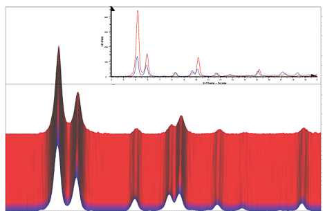
Figure 4. Thermodiffractiongram of species 4 , highlighting the substantial constancy of its XRPD pattern, when heated, in air, from rt (blue trace) to 410 °C. The upper insert shows the relative changes of peak intensities due to extraframework water elimination.
