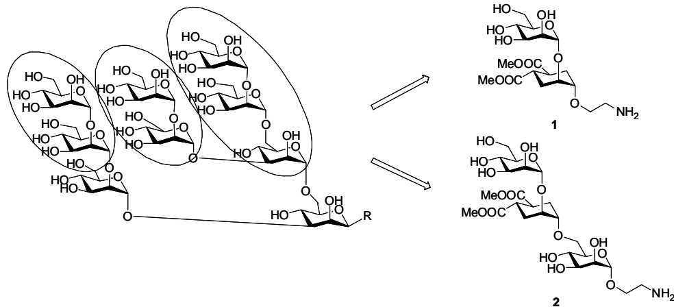
Figure 1. Glycomimetics structures 1 and 2 based on the high-mannose oligosaccharide.
