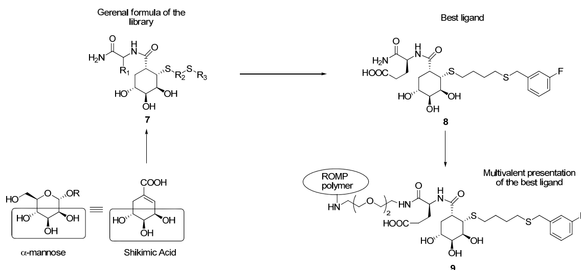
Figure 4. Kiessling shikimic acid-derived glycomimetic strategy to prepare DC-SIGN inhibitors.
