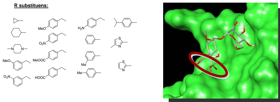
Figure 3. Design of a library of bis-amides based on the structure of glycomimetic 1 .
