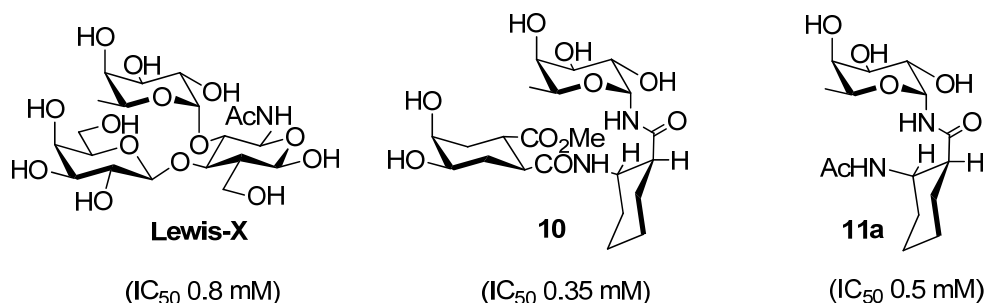
Figure 5. First series of Fucose-based DC-SIGN inhibitors.
