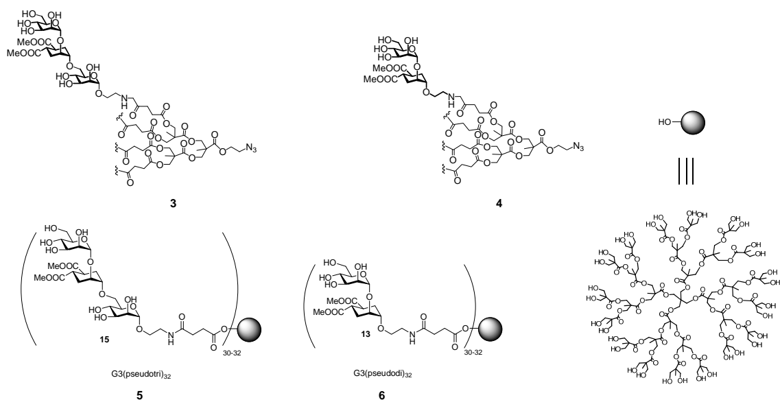
Figure 2. Multivalent presentation of glycomimetics 1 and 2 using dendrons ( 3 , 4 ) and dendrimers ( 5 , 6 ) scaffolds.
