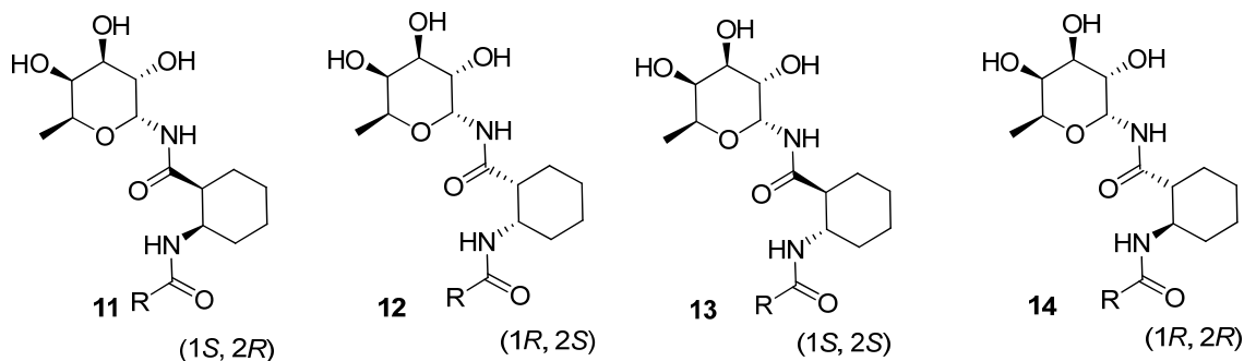
Figure 6. Second generation of Fucose-based ligands for DC-SIGN.
