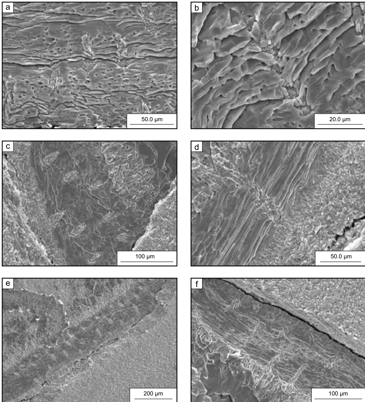
Plate 1: Khuff Formation brachiopods from Saudi Arabia showing well-preserved non-luminescent secondary layer fibres in Omanilasma husseinii from sample level KH0211: (a) specimen KH0211-2; (b) specimen KH0211-7; (c) specimen KH0211-8; (d) specimen KH0211-8; (e) specimen KH0211-9; (f) specimen KH0211-11.
