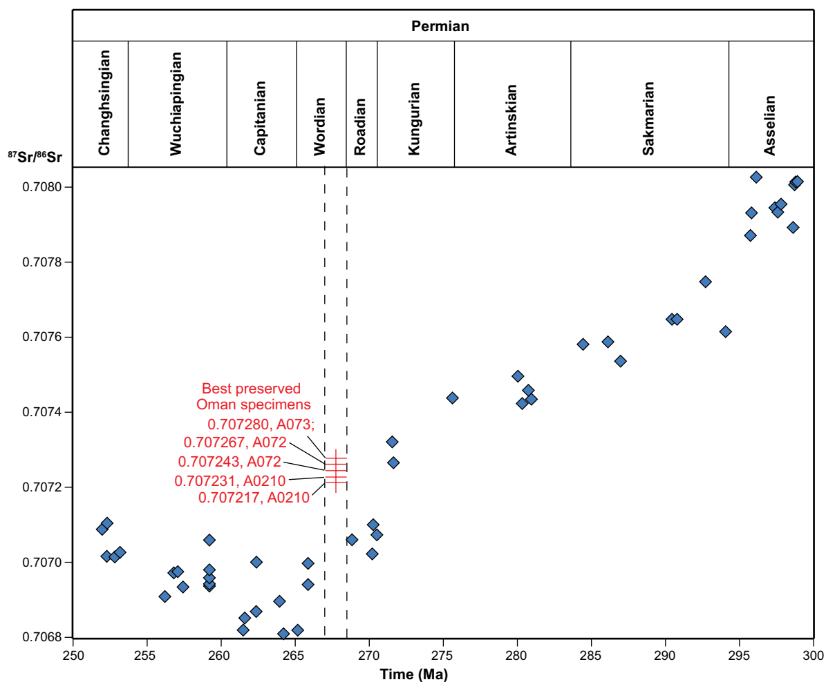
Figure 4: ^{87}\text{Sr}/^{86}\text{Sr} from Korte et al. (2006), blue diamonds; and Oman ^{87}\text{Sr}/^{86}\text{Sr} data, red crosses. Dates from ICS ( http://www.stratigraphy.org/ ). The ^{87}\text{Sr}/^{86}\text{Sr} from Oman brachiopod horizons are plotted within the range of the early Wordian in accordance with their biostratigraphic age.
