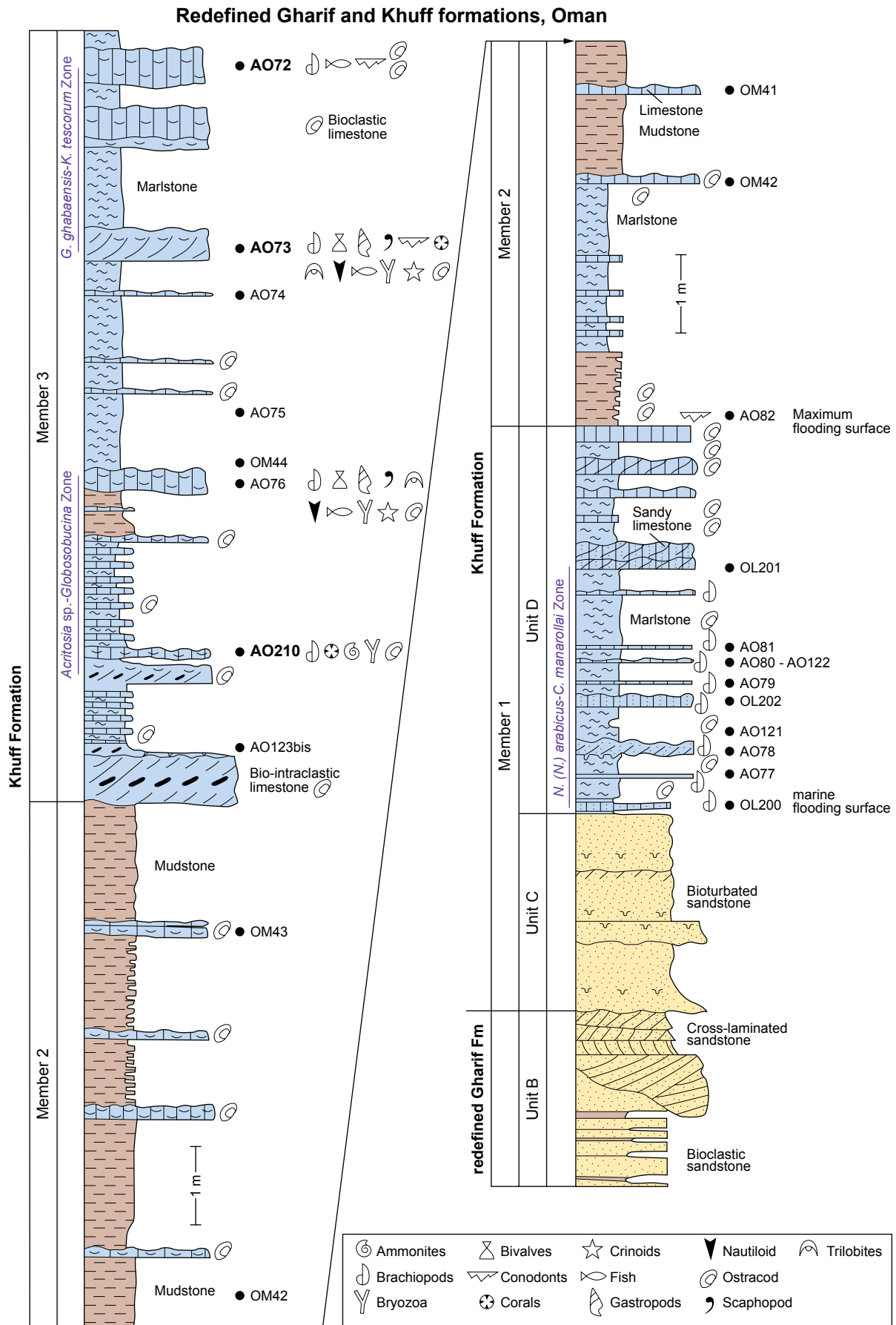
Figure 2: Graphic log of the three members of the Khuff Formation in Interior Oman, section K7 at 21°02'30"N-57°42'00"E, showing the stratigraphic position of the brachiopod horizons in bold (after Angiolini et al., 2004).
