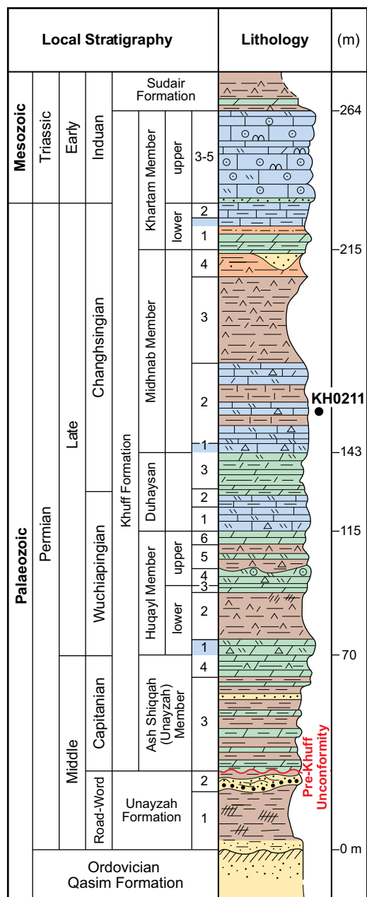
Figure 3: Graphic log of the Khuff Formation in the Buraydah Quadrangle, northern Central Saudi Arabia, showing the location of the brachiopods collected in pebbly bioclastic calcarenite in the Midhnab Member (modified from Vaslet et al., 2005; Angiolini et al., 2006).
