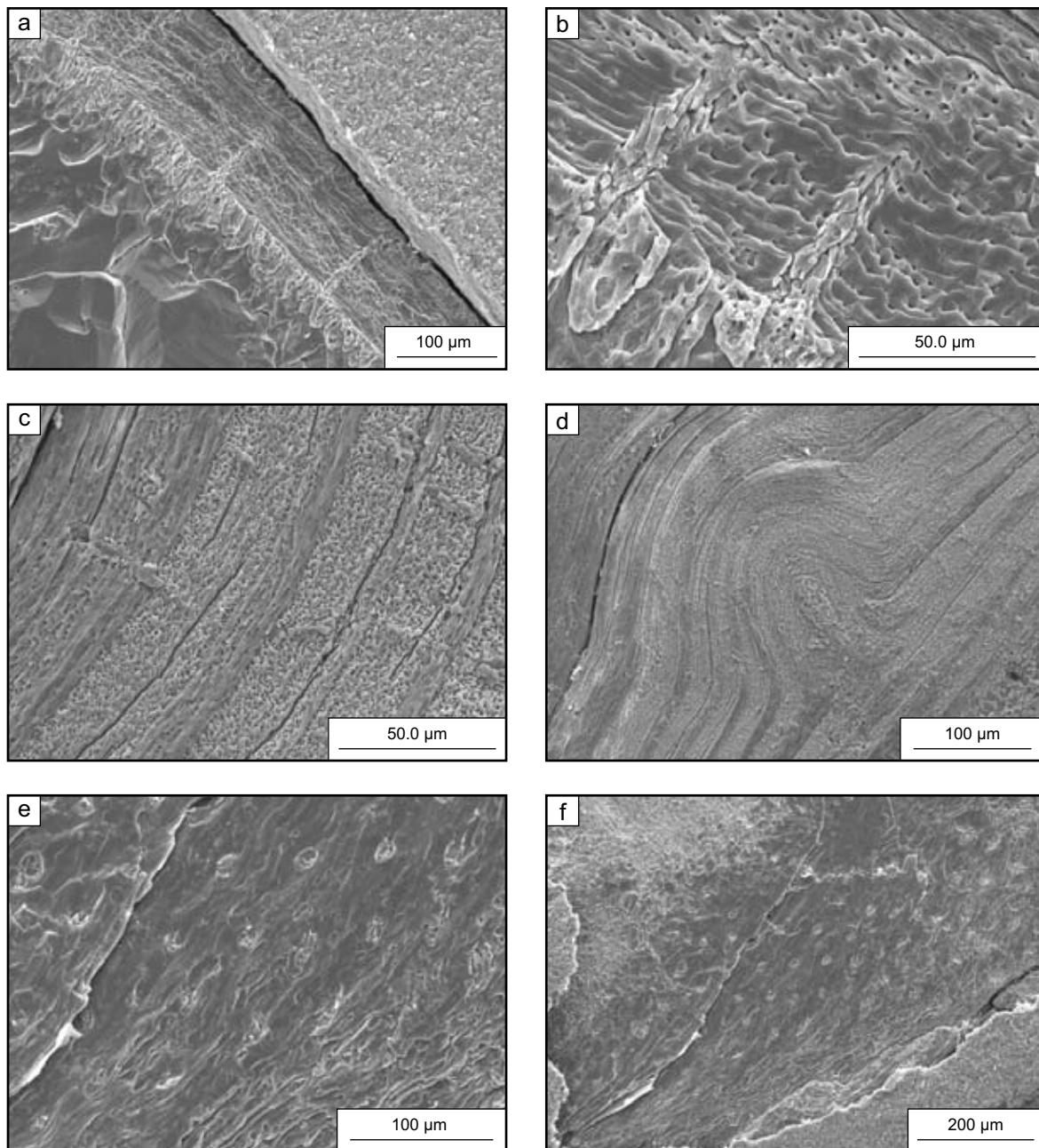
Plate 2: (a) and (b): Khuff Formation brachiopods from Saudi Arabia showing well-preserved non-luminescent secondary layer fibres in Omanilasma husseinii from sample level KH0211: (a) specimen KH0211-11; (b) specimen KH0211-11. (c) and (d) Oman specimens of Juresania omanensis characterised by a secondary laminar shell. These tend to be more easily altered around the hollow base of a spine and appear cathodoluminescent: (c) specimen AO72-16; (d) specimen AO72-16. (e) and (f) Well-preserved non-luminescent secondary shell of Oman specimens of O. husseinii which is much thicker than conspecific Saudi Arabia specimens, reaching thicknesses of more than 500 \mu\text{m} . The secondary layer fibres have a keel and saddle profile with a thickness of 3–5 \mu\text{m} and are deflected around larger punctae (diameter 30–45 \mu\text{m} ): (e) specimen AO73-39. (f) specimen AO73-39.
