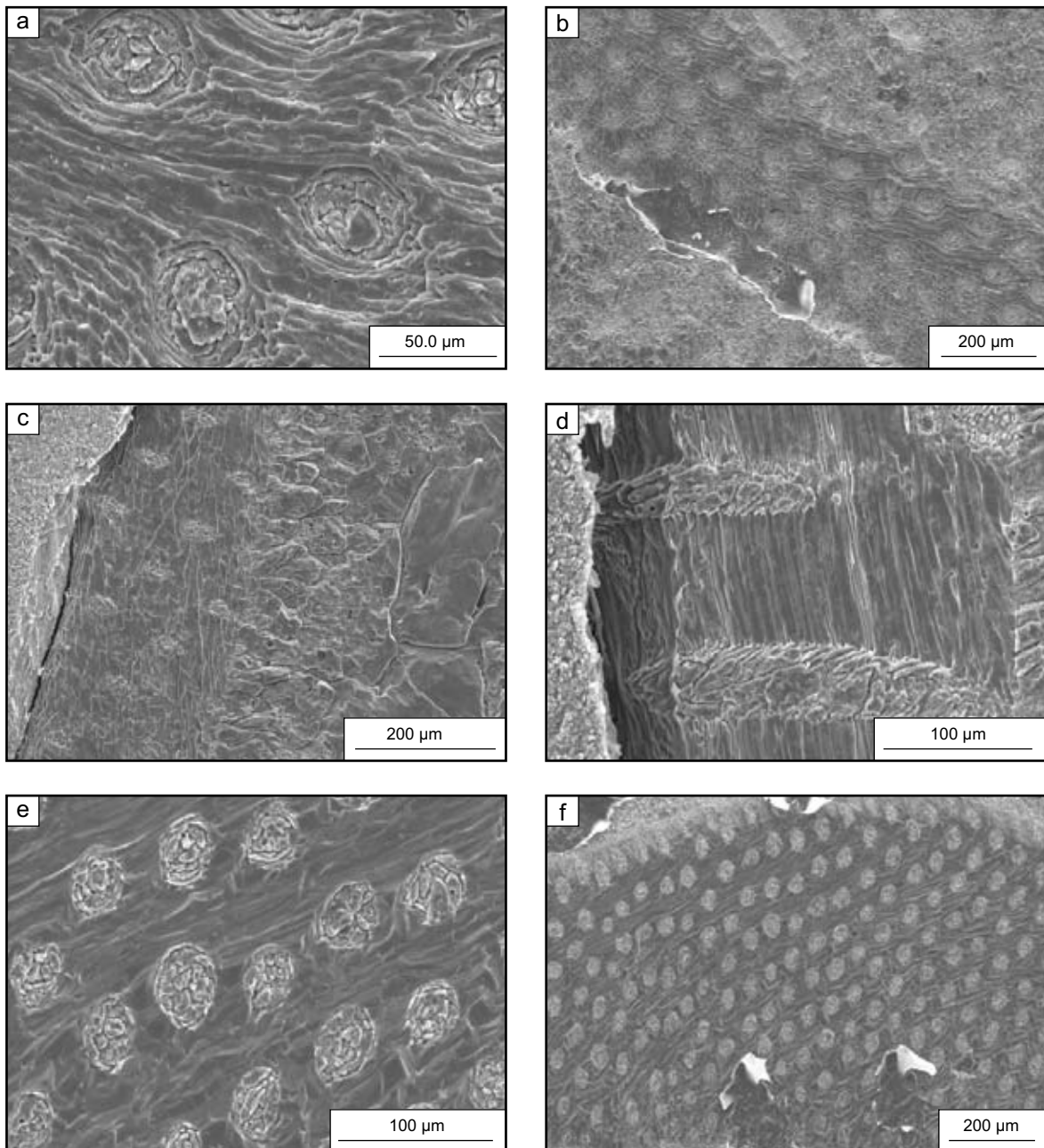
Plate 3: Oman specimens of O. husseini . (a) specimen AO73-44; (b) specimen AO73-44; (c) specimen AO210-3; (d) specimen AO210-9; (e) specimen AO210-25; (f) specimen AO210-25.
