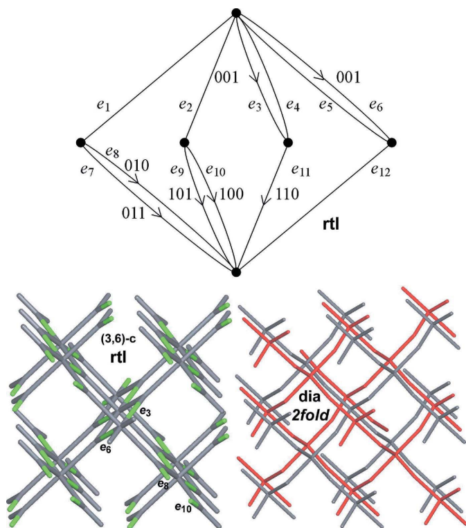
Figure 7 (Top) Labelled quotient graph of rtl , (bottom left) representation of rtl and (bottom right) twofold dia obtained after deleting the edge set \mathcal{S}_2 = \{e_3, e_6, e_8, e_{10}\} enhanced in green in rtl .
