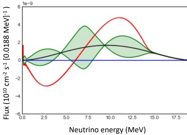
FIG. 4 The hep spectrum is in black, and the uncertainties in ^8\text{B} from Longfellow et al. (Longfellow et al. , 2023) span the region between the green lines. The red line indicates the difference between Longfellow et al. and Winter et al. (Winter et al. , 2006) deduced ^8\text{B} spectra. The hep spectrum is used here as a convenient metric for the size of the uncertainties in the ^8\text{B} spectrum.
