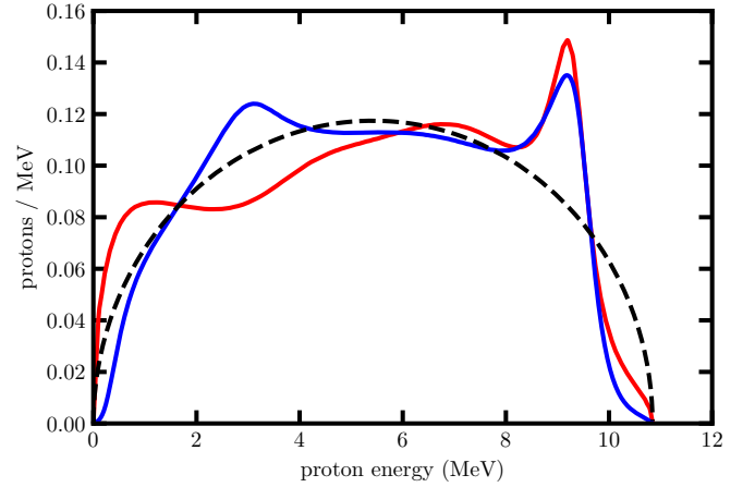
FIG. 6 Calculated proton energy spectra in the c.m. frame for the {}^3\text{He}({}^3\text{He}, 2p){}^4\text{He} reaction at E_{\text{c.m.}} = 165 keV. The solid red and blue curves are models 1 and 2, respectively, from Fig. 3(a) of Zylstra et al. (2017) . The black dashed curve is the elliptical spectrum. The spectra are normalized to unit area.
