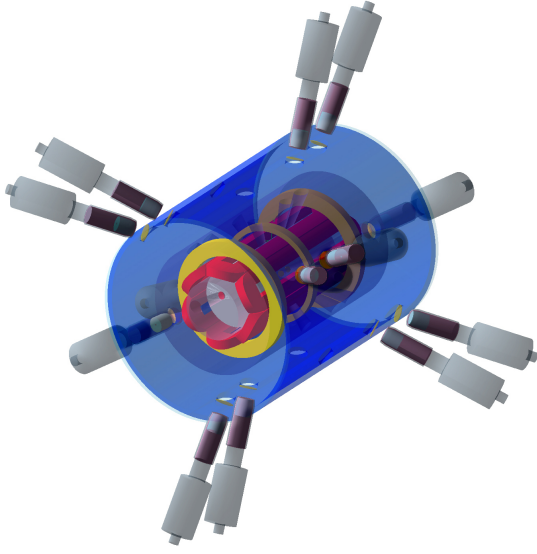
FIG. 14 Schematic drawing of the PANDORA trap with holes to house the HPGe detectors. (credit: Domenico Santonocito).
