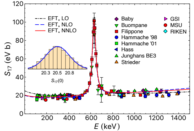
FIG. 8 Astrophysical S-factor for {}^7\text{Be}(p, \gamma){}^8\text{B} . Data with E \leq 1250 keV were included in the Bayesian fits shown here, which use the halo EFT of Higa et al. (2022) that includes an excited {}^7\text{Be} component. The dot-dashed (black) curve is the LO calculation, the dashed (blue) curve is NLO, and the solid (red) curve is NNLO. The inset shows the posterior probability distribution function for S_{17}(0) in eV b. The median as well as the 16th and 84th percentiles of the distribution are specified.
