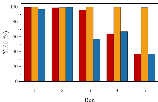
Fig. 8. Yield in aniline in the reduction of nitrobenzene to aniline with 10 % excess hydrazine catalyzed by GO@Ni (red, 15 mol%), RGO@Ni (yellow, 15 mol%) and Ni (blue, 15 mol%) at 20 °C under N 2 atmosphere.
