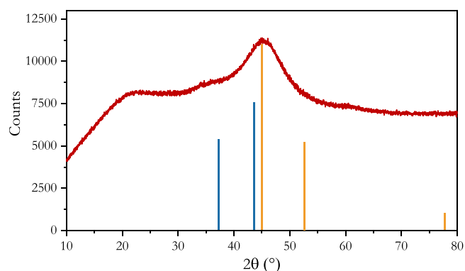
Fig. 3. XRD of RGO@Ni (red curve), Ni (yellow peaks) and NiO (blue peaks).
