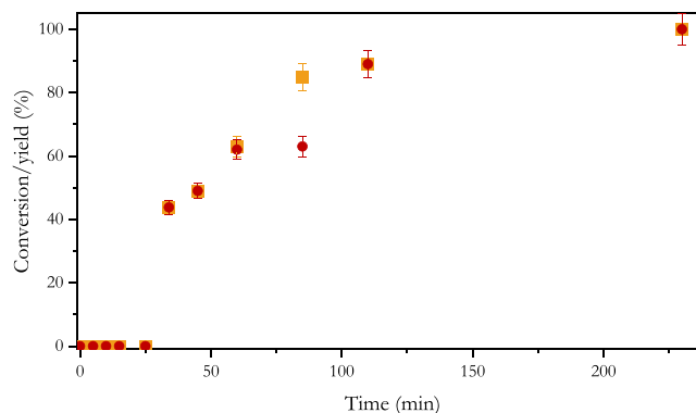
Fig. 7. Yield in aniline (red circles) and substrate conversion (yellow squares) in the reduction of nitrobenzene with hydrazine catalyzed by RGO@Ni (15 mol %) at 35 °C under N 2 atmosphere.
