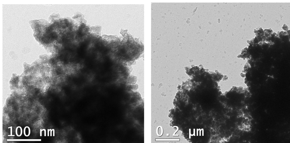
Fig. 4. TEM photographs of RGO@Ni at low magnification degrees.
