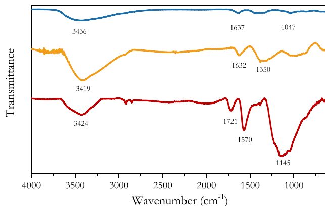
Fig. 1. FTIR spectra of GO (red), GO@Ni (yellow) and RGO@Ni (blue).
