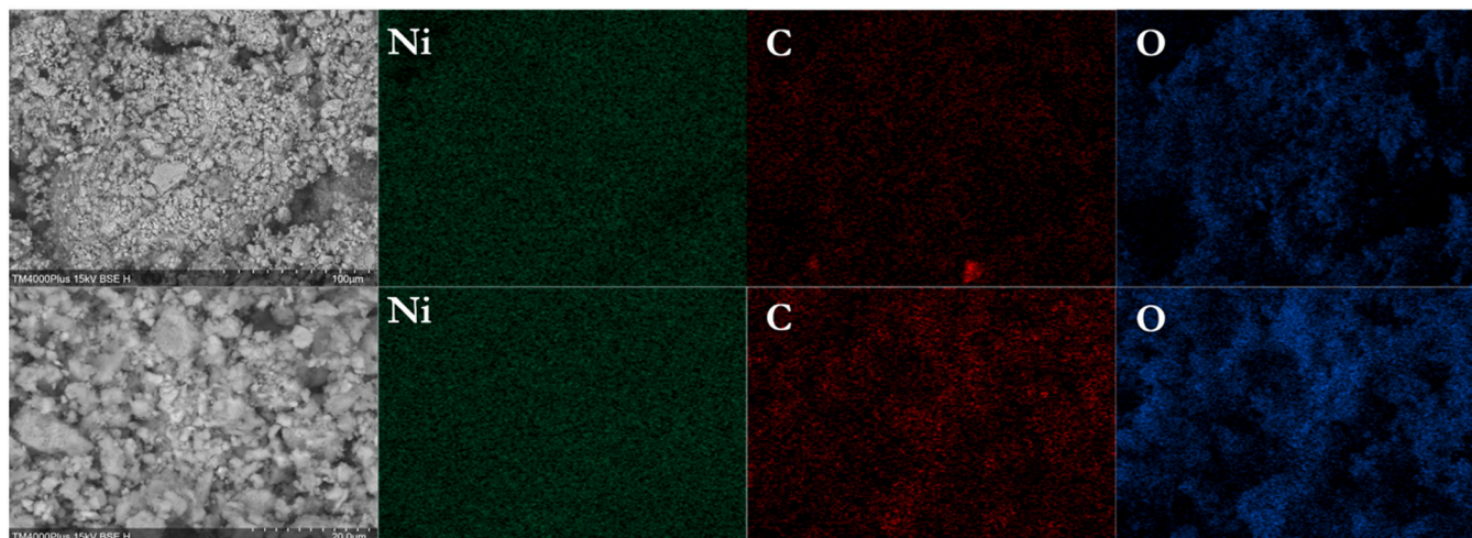
Fig. 6. SEM photographs and elemental maps of RGO@Ni at different magnification levels.
