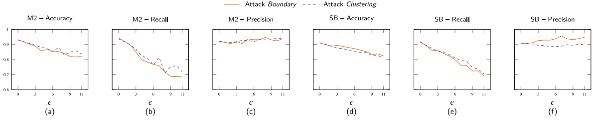
Fig. 3. Impact of poisoning attacks against the vanilla monolithic model, using datasets M2 and SB and varying the percentage of poisoned data points \epsilon .
