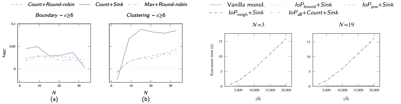
Fig. 7. Average \Delta on dataset SB under attacks Boundary and Clustering with \epsilon \geq 6 , varying N .
