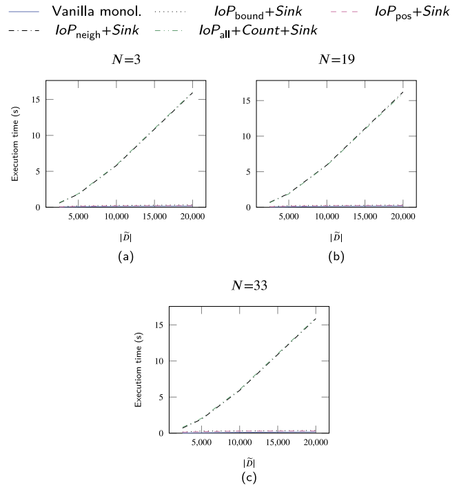
Fig. 8. Performance of our technique varying dataset cardinality |\tilde{D}| (oversampled from dataset SB under Boundary with \epsilon = 6 ).
