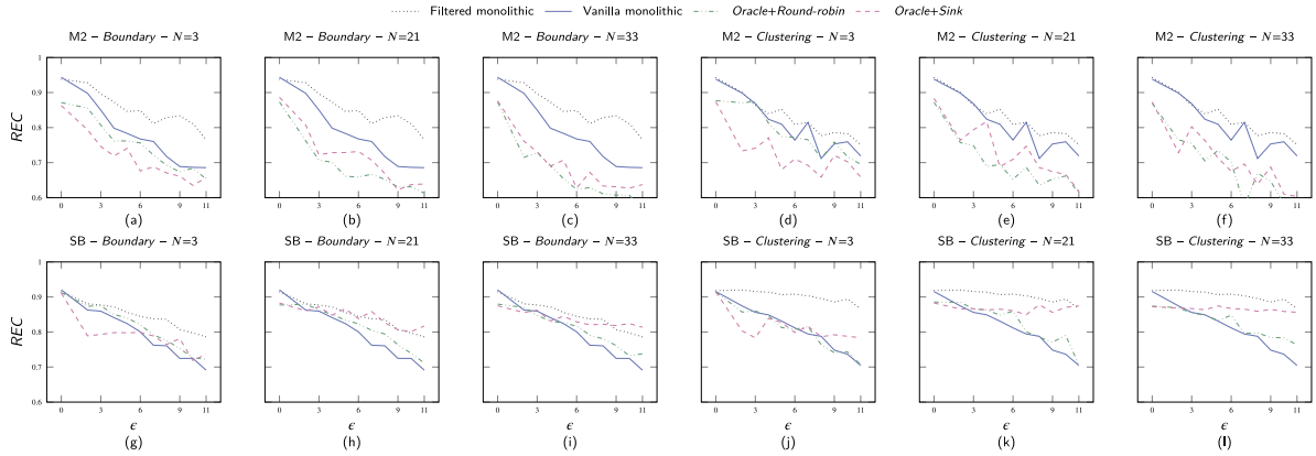
Fig. 4. Impact of poisoning attacks against vanilla and filtered monolithic models and risk oracle pipelines, varying datasets M2 and SB and percentage of poisoned data points \epsilon .
