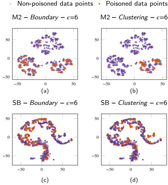
Fig. 5. Dimension-reduced datasets M2 and SB. (For interpretation of the references to color in this figure legend, the reader is referred to the web version of this article.)
