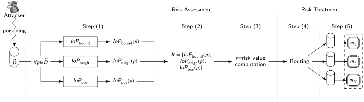
Fig. 1. Overview of our risk-based ensemble technique.
