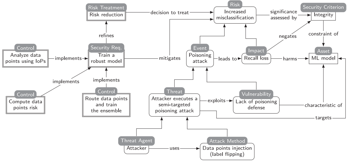
Fig. 2. Conceptual modeling of our risk-based approach according to the Information System Security Risk (ISSRM) domain model (Matulevičius, 2017). Straight-corners rectangles depict asset concepts, rounded-corners rectangles risk assessment concepts, while double-line rectangles risk treatment concepts. We report the asset “ML model” without distinguishing between IS and Business assets.
