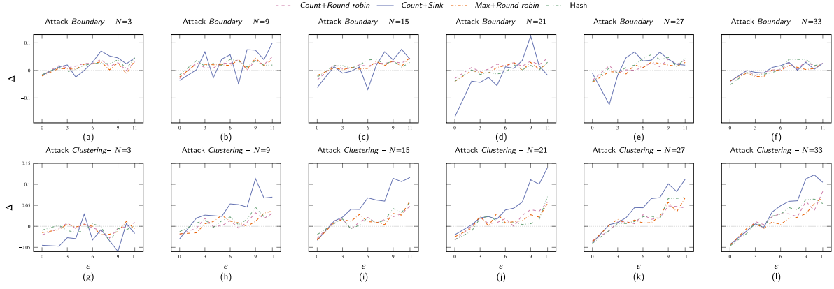
Fig. 6. \Delta of risk pipelines varying percentage of poisoned data points \epsilon .
