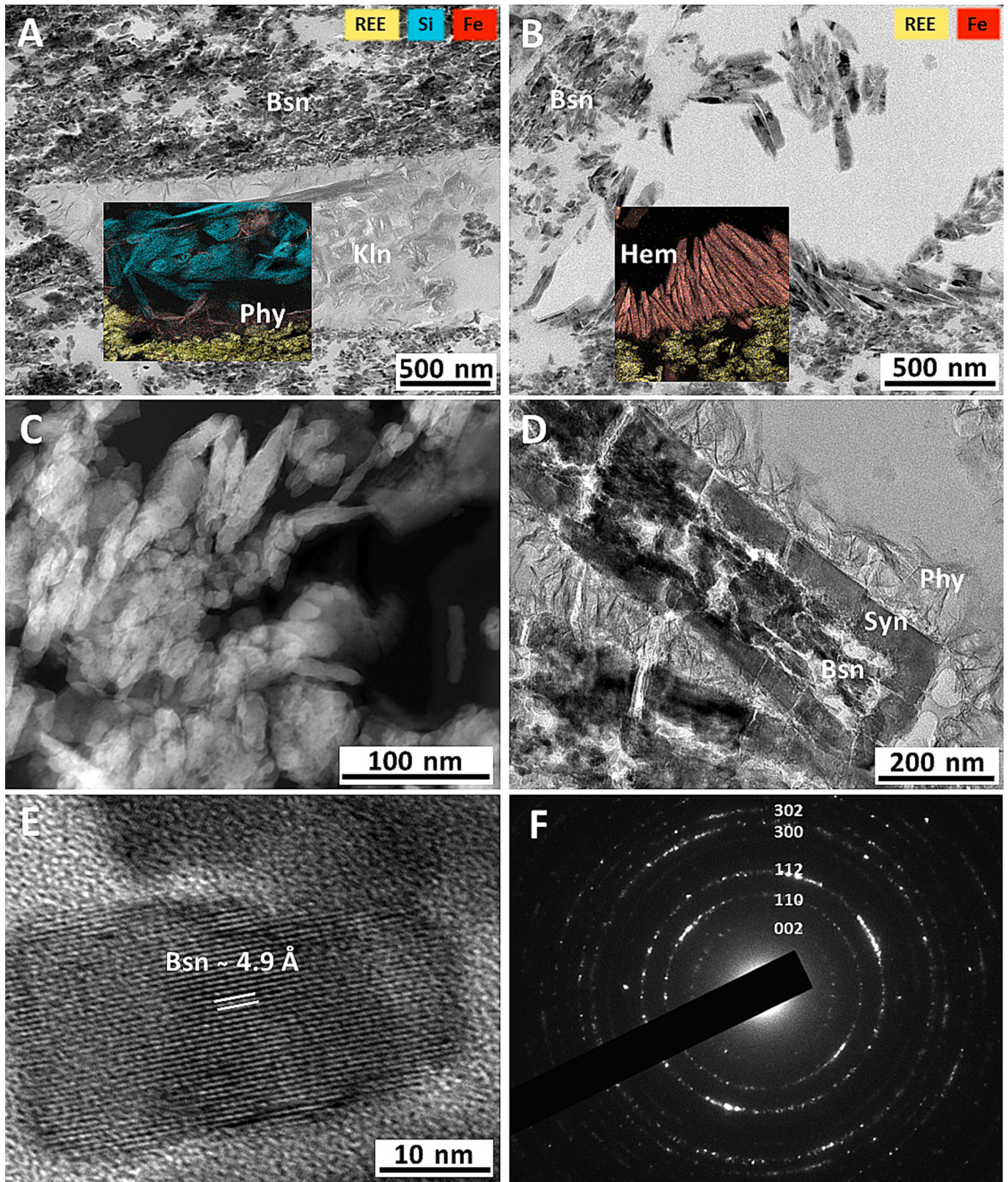
Fig. 9. Bright field TEM images with superimposed TEM-EDS maps showing: A) and B) the nanostructure of bastnäsité-(Nd) in which bastnäsité nanocrystals (Bsn) are intergrown with phyllosilicates (Phy), kaolinite-like (Kln) and hematite (Hem); C) HAADF STEM image showing the spindle shape of bastnäsité nanocrystals. D) "scaffold" nanostructure with bastnäsité nanocrystals walled by synchysite-(Ce) (Syn) and phyllosilicates (Phy). E) Lattice fringe image of bastnäsité-(Nd) showing a constant \sim 4.9 Å spacing. F) SAED patterns of bastnäsité nanocrystals showing the typical diffraction rings of polycrystalline materials (main rings indexed).
