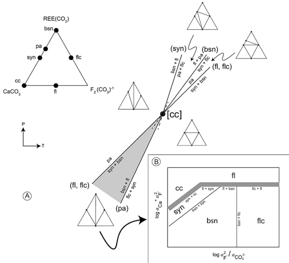
Fig. 10. (A) P - T net around the bundle [cc] showing phase relations at low- T and low- P in the \text{REE}(\text{CO}_3)\text{F}-\text{CaCO}_3-\text{F}_2(\text{CO}_3)_{-1} system (bsn = bastnäsite, syn = synchysite, fl = fluorite, flc = fluocerite, cc = calcite, pa = parisite). (B) Schematic isobaric-isothermal \log(a_{\text{Ca}^{2+}} \cdot a_{\text{F}^{-}}^2) vs. \log(a_{\text{F}^{-}}^2 / a_{\text{CO}_3^{2-}}) diagram corresponding to the shaded divariant phase field in (A). It can be seen that crystallization may switch from synchysite to bastnäsite by decreasing the activity of \text{Ca}^{2+} and \text{F}^{-} while keeping constant the a_{\text{F}^{-}}^2 / a_{\text{CO}_3^{2-}} ratio, and vice versa (from Williams-Jones and Wood, 1992, modified).
