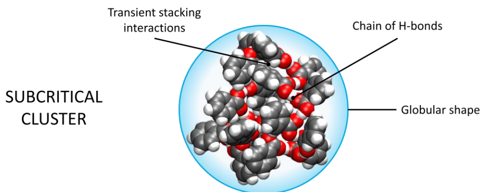
Figure 1. Subcritical cluster of benzoic acid consisting of 17 molecules, with a maximum lifetime exceeding 130 ps.
