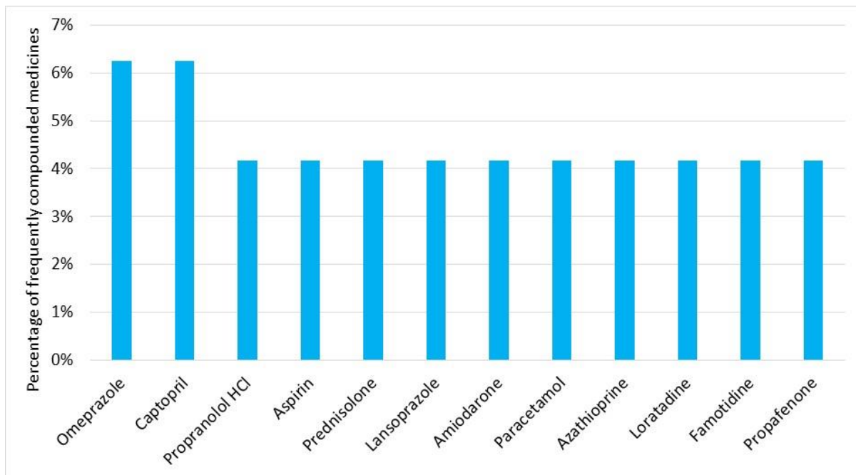
Fig. 2f South East Asia
