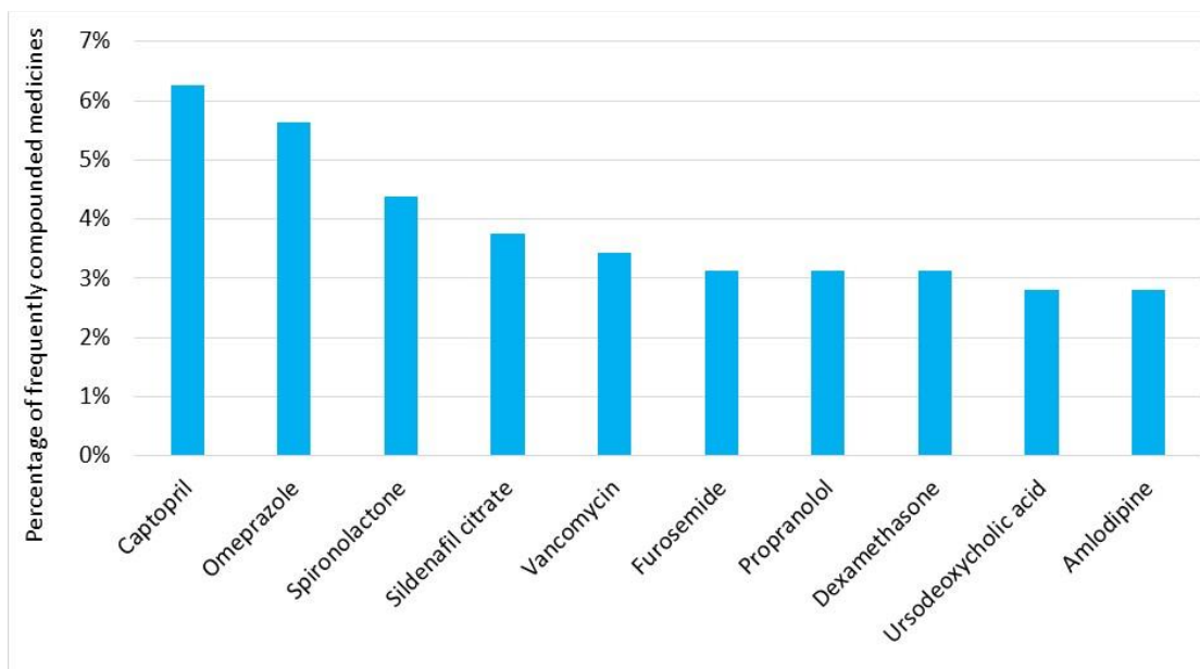
Fig. 2b Eastern Mediterranean
