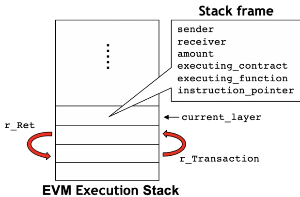
Figure 1: Ethereum VM Modeling.
