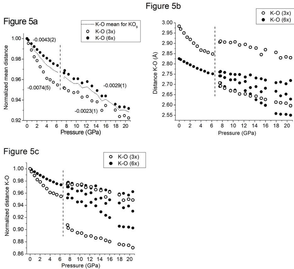
Fig. 5 The bond lengths within the ninefold coordinated K site in synthetic bütschliite \text{K}_2\text{Ca}(\text{CO}_3)_2 : pressure evolution of (a) the normalized average K-O bond distances; (b) the individual K-O bond distances, and (c) and their normalized values. The trigonal-to-monoclinic phase transition pressure is marked by dash line
