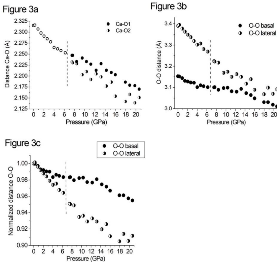
Fig. 3 Main interatomic distances and bond lengths of the octahedrally coordinated Ca in synthetic bütschliite K_2Ca(CO_3)_2 : pressure dependencies of (a) the cation-oxygen bond distances, (b) the O-O distances corresponding to the octahedral basal and lateral edges, and (c) and their normalized values. The trigonal-to-monoclinic phase transition pressure is marked by dash line
