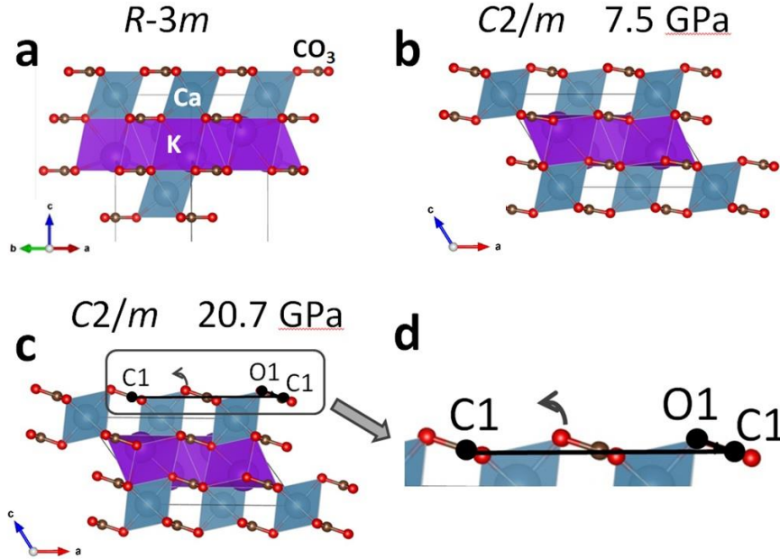
3 4 Fig. 1 Crystal structure of the \text{K}_2\text{Ca}(\text{CO}_3)_2 bütschliite polymorphs as derived from the single-crystal data 5 collected at (a) ambient pressure, (b) 7.52 GPa and (c) 20.65 GPa. The space group and pressure value 6 are indicated on the top of each figure. The cation sites K (violet) and Ca (blue), and the carbonate groups 7 ( \text{CO}_3 ) are labeled accordingly. In the monoclinic structure the coordination around the K atoms is 8 displayed as \text{KO}_9 instead of \text{KO}_{11} polyhedra for an easier comparison with the trigonal structure. The 9 solid black line in (c) marks the angle \text{O1-C1-C1} , enlarged in (d), which accounts for the coupled 10 polyhedral rotation (indicated by arrow) of \text{CO}_3 and \text{CaO}_6 building units. The structure is visualized using 11 the program VESTA 3 (Momma and Izumi 2011) 12
