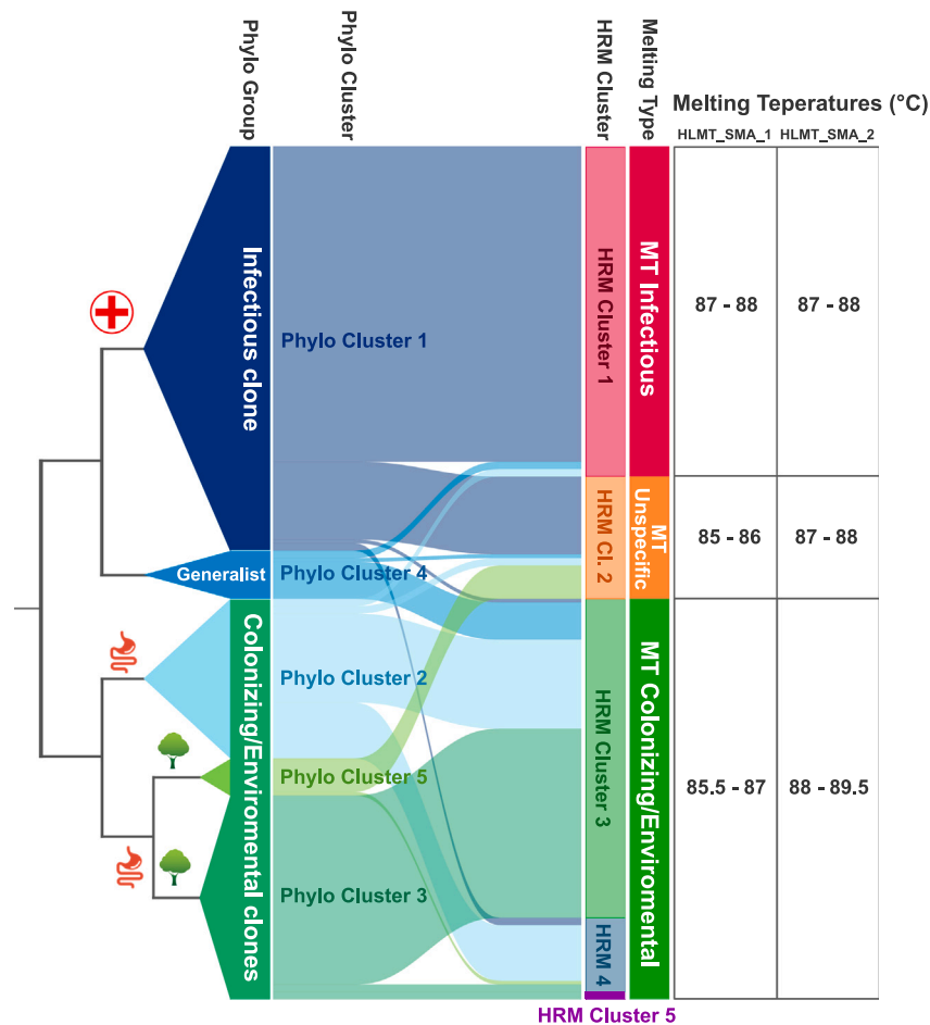
Figure 2. WGS-based typing vs. HRM-based typing
