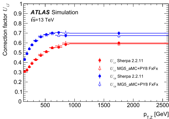
Fig. 7. The value of the correction factor, U_{i,\ell} , as a function of p_{T,Z} for both the Z \rightarrow ee (in red) and Z \rightarrow \mu\mu (in blue) regions. Shown in solid dots is the correction as determined with SHERPA 2.2.11 simulations and in open triangles that determined with MG5_AMC+Py8 FxFx simulations. Only the Monte Carlo statistical uncertainties are shown.
