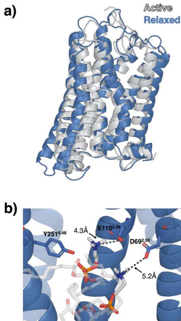
Figure 1: OR51E2 from simulations without ions in the binding pocket. (a) Superposition of the cluster centroid obtained from the five trajectories (blue) started from the cryoEM structure in its active state (white), evidencing the widening of the TM6-TM7 interface. (b) Detail of the ion binding pocket, highlighting the interaction between the charged residues D69 2,50 and E110 3,39 and the two POPC headgroups entering the receptor bundle. Additionally, Y251 6,48 is oriented towards the ion binding pocket. Hydrogen atoms have been omitted for clarity, and the distances refer to the frame shown.
