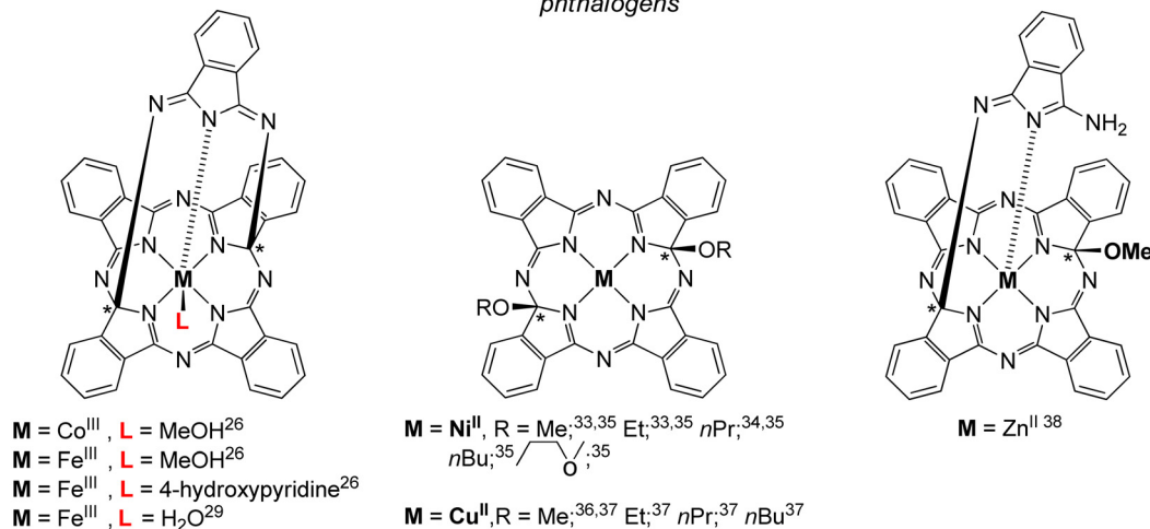
Fig. 1 Chemical structures of crystallographically characterized phthalogens. 11 The sign * indicate asymmetrically substituted carbon atoms but refer to racemic mixtures.
