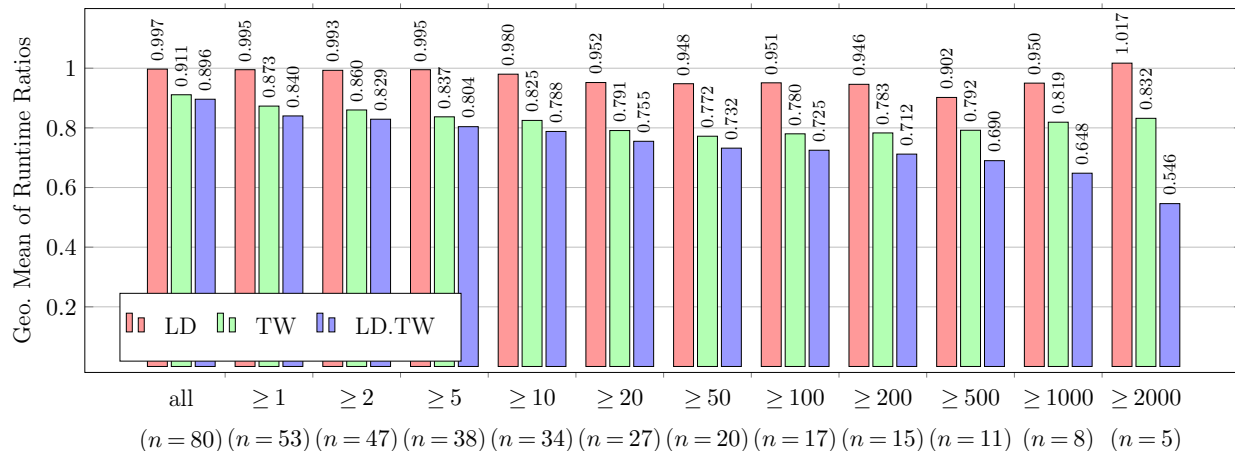
Figure 2 Geometric mean of the computation time ratios w.r.t. to the baseline setting AF (arc fixing) for the resource-window reduction settings LD, TW, and LD.TW for the VRPTW; results are grouped according to running times where \geq rt indicates that only instances with a computation time t_{AF} of at least rt are considered.
