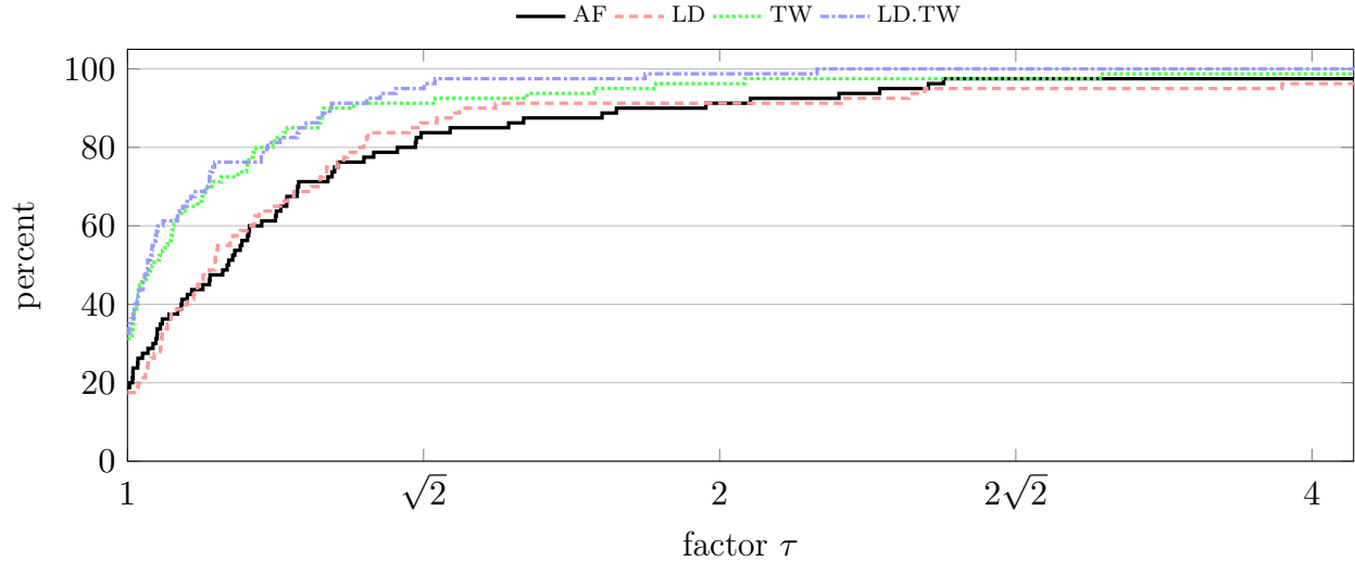
Figure 3 Performance profiles \rho_X(\tau) for the four computational settings X \in \{\text{AF}, \text{LD}, \text{TW}, \text{LD.TW}\} . Note that the logarithmic scale on the axis of abscissae ( \tau values) is considered.
