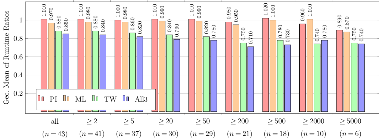
Figure 4 Geometric mean of the computation time ratios w.r.t. to the baseline setting AF (arc fixing) for the resource-window reduction settings PI, ML, TW, and All3 for the VRPSDPTW; results are grouped according to running times where \geq rt indicates that only instances with a computation time t_{AF} of at least rt are considered.
