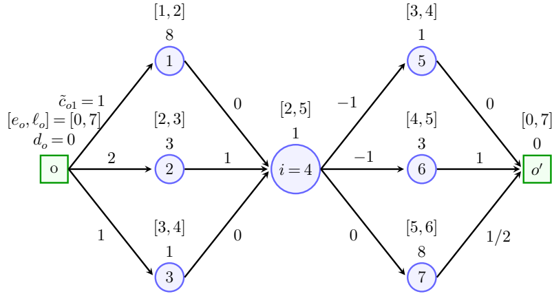
(a) Network (V, A) with reduced costs on arcs and time windows and demands on vertices; all travel times are 1.
