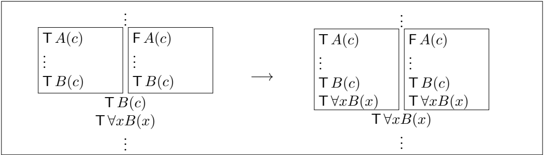
Figure 7: The result of this transformation shows an application of the liberalized \text{T}\forall I rule.
