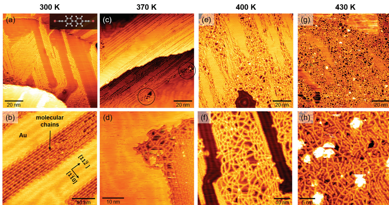
Fig. 1 STM images of on-surface synthesized sp - sp^2 C polymers. 100 \times 100 \text{ nm}^2 images are reported in the upper row, and smaller-scale ones in the lower row. (a) STM image of the sample observed after deposition of bBEBP molecules on Au(111) at room temperature. Inset: Ball-and-stick structure of a bBEBP molecule, where red dots represent Br atoms, grey dots C atoms and white dots H atoms. (b) Close-up of a surface region showing linear wires aligned along the [11\bar{2}] Au(111) direction. (c) and (d) STM images taken after annealing at 370 K. Black circles in (c) indicate locally disordered regions, as that shown in (d) at higher resolution. (e) and (f) STM images taken after annealing at 400 K. (g) and (h) STM images taken after annealing at 430 K.
