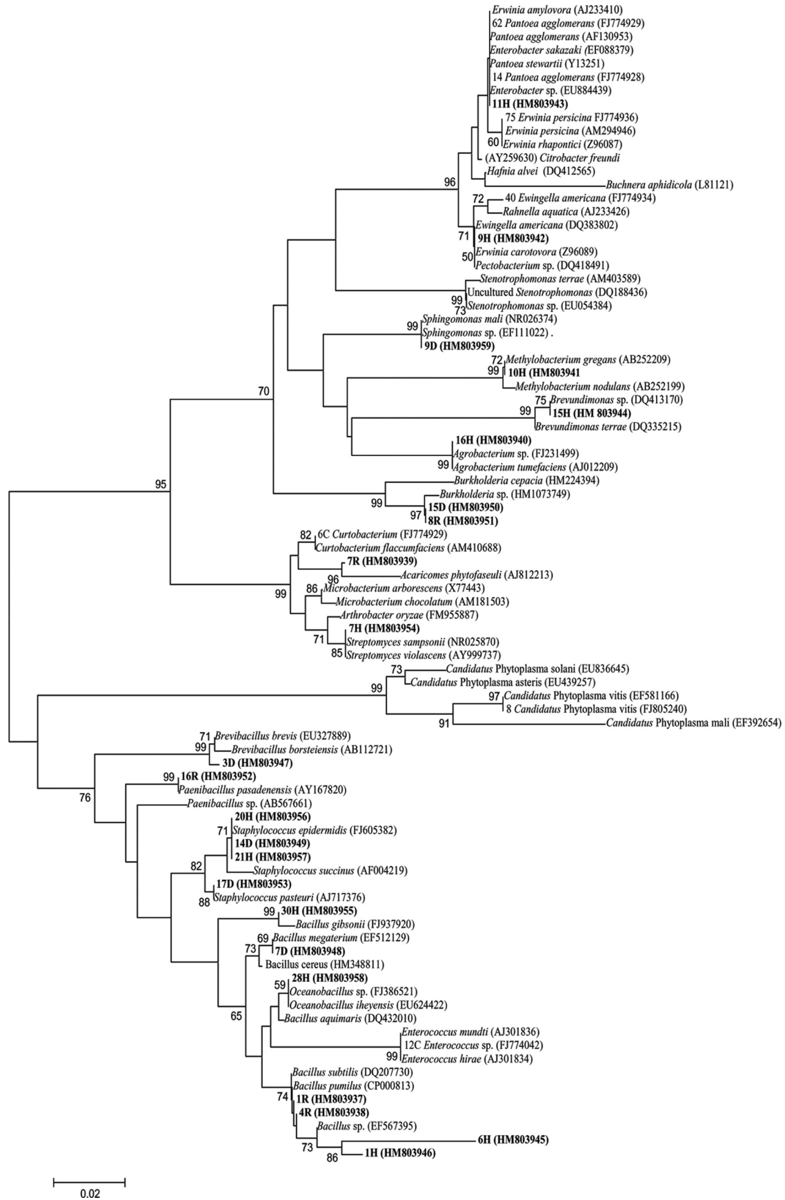
FIG. 2. Phylogenetic relationships based on partial 16S rRNA gene sequences obtained from the endophytic bacteria associated with grapevine tissues (this work) and closely related sequences retrieved from GenBank. Bootstrap values are displayed at tree nodes. GenBank accession numbers of nucleotide sequences are shown along with the name of the bacterial species.
