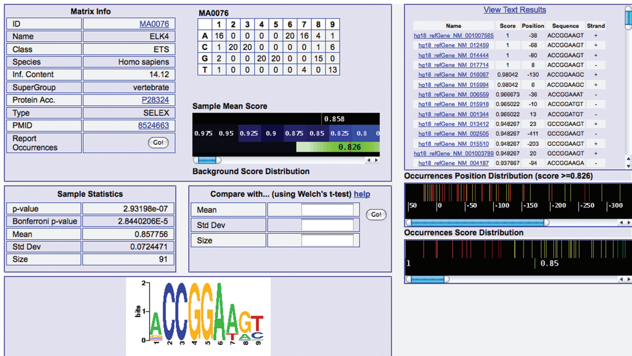
Figure 4. Example of the detailed information displayed by Pscan concerning JASPAR motif ELK4, with (left) matrix, logo (bottom left), cross-references, average score in the input set compared to the background mean and standard deviation (green area). Under these pieces of information, the interface shows the statistics for the matrix on the input set, together with an input form for the comparison of the results on different input sets. On the right, there is the list of best occurrences in each input promoter, with gene name, oligo score, position with respect to the TSS of the gene, oligo sequence and strand. Notice how the best occurrences (with score higher than the background average) are mostly located in the core promoter area (-100, +50).
