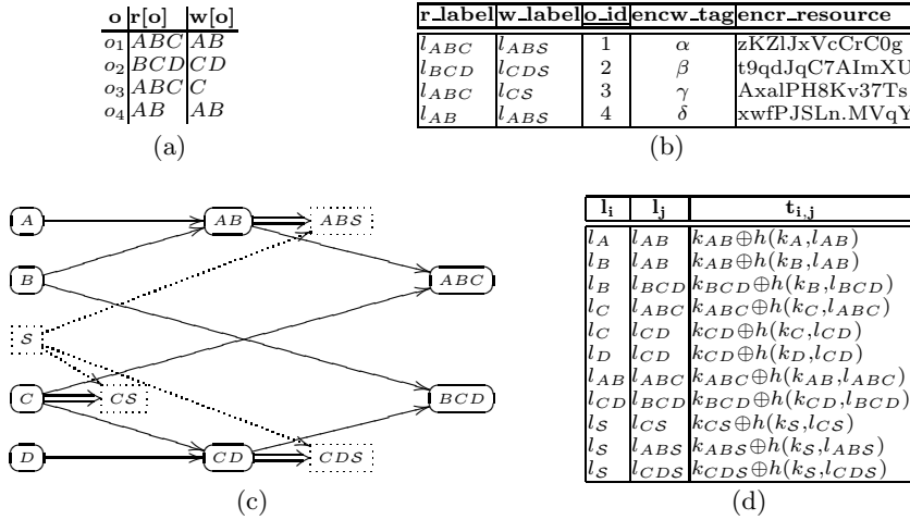
Fig. 3. An example of read and write acs (a), encrypted resources (b), key derivation structure (c), and tokens (d)
