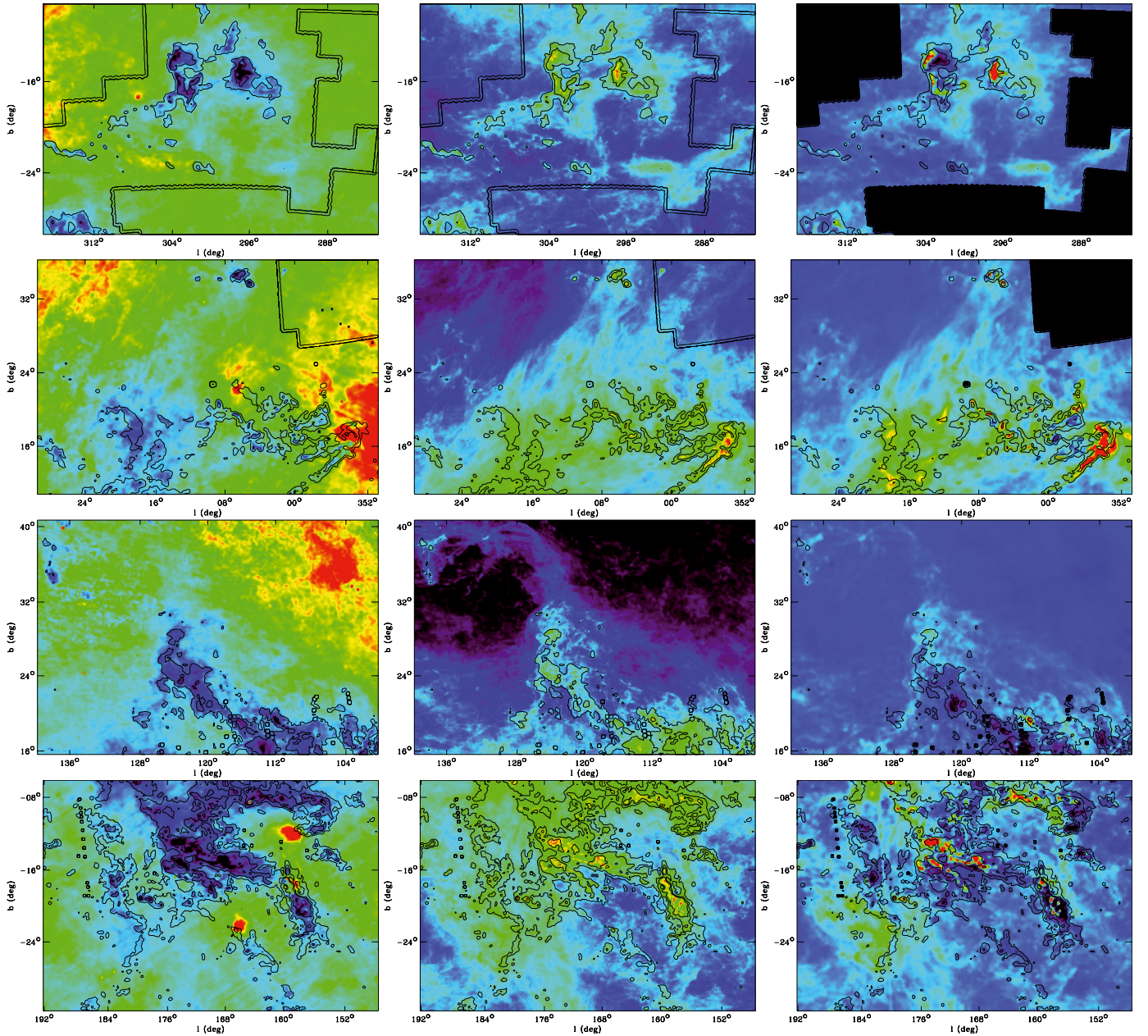
Fig. 4. Details of the dust temperature ( left column ), dust optical depth at 857 GHz ( central column ) and dark gas column density ( right column ) for the Chamaleon (first line), Aquila-Ophiuchus flare (second line), Polaris flare (third line) and Taurus (fourth line). The temperature and optical depth maps are shown in log scale with a colour scale ranging from 15 K (black) to 20 K (red) and 1 \times 10^{-5} (black) to 3 \times 10^{-3} (red) respectively. The dark gas column density derived from the optical depth at 857 GHz (see Sect. 4) and is shown in linear scale with a colour scale ranging from -3 (black) to 7 \times 10^{21} H cm ^{-2} (red). The contours show the ^{12}\text{CO}(J = 1 \rightarrow 0) integrated intensity at 2, 10 and 20 K km s ^{-1} . The double line shows the limit of the CO surveys.
