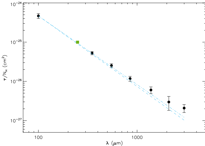
Fig. 7. Dust optical depth derived from this study using the IRAS and Planck -HFI frequencies. The square symbol shows the emissivity at 250\mu\text{m} derived by Boulanger et al. (1996). The dash and dash-dot lines show a power law emissivity with \lambda^{-1.8} and \lambda^{-1.75} respectively, normalized to the data at 100\mu\text{m} . The error bars shown are \pm 1\sigma .
