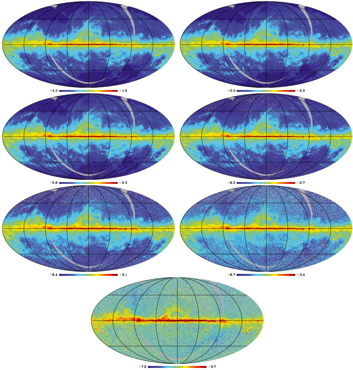
Fig. 5. Maps of the dust optical depths on a log scale, in the IRAS 100 \mu\text{m} (first row left) and Planck -HFI bands at 857 (first row right), 545 (second row left), 353 (second row right), 217 (third row left), 143 (third row right) and 100 GHz (fourth row). All maps are shown in Galactic coordinates with the Galactic centre at the centre of the image. The missing data in all images correspond to the IRAS gaps. The upper and lower bounds of the colour scale are set to \tau_{\text{min}} = 5 \times 10^{-5} \times (\lambda/100 \mu\text{m})^{-1.8} and \tau_{\text{max}} = 10^{-2} \times (\lambda/100 \mu\text{m})^{-1.8} respectively.
