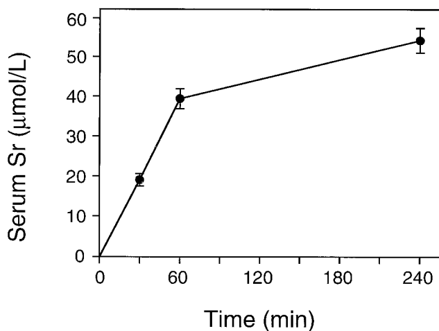
Fig. 1. Sr concentrations in serum measured 30, 60, and 240 min after an oral load of 30.2 \mu mol/kg body wt (2.65 mg/kg body wt; see Methods).
