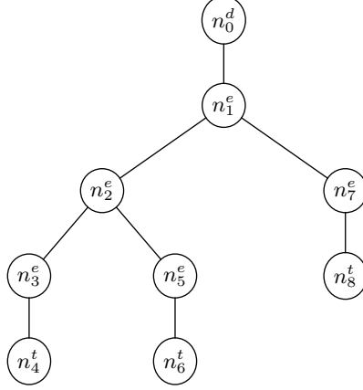
Fig. 3. XML tree of Example 2.1
