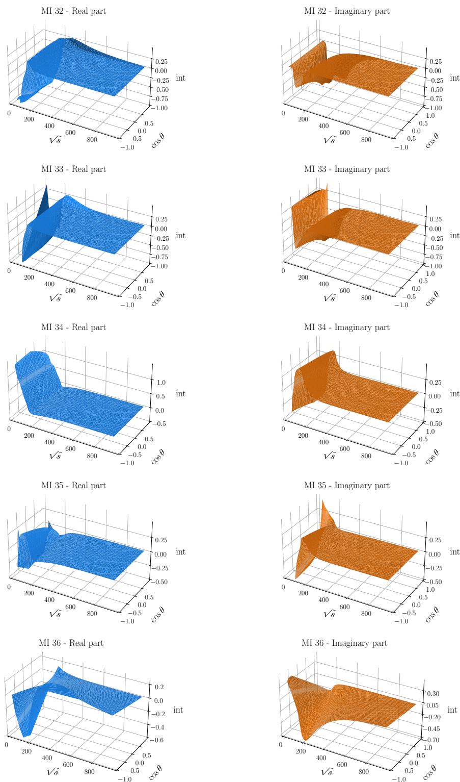
Figure 4. Real (left column) and imaginary (right column) parts of the \epsilon^0 coefficient of the two-mass MIs labeled 32 to 36 in ref. [66].
