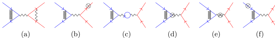
Figure 2. Sample Feynman diagrams of factorisable corrections, including one-loop counterterm corrections.
