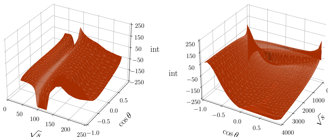
Figure 5. The contributions from all the vertex and box Feynman diagrams to the \mathcal{O}(\alpha_s) correction to the finite hard function, in two different invariant mass ranges, as a function of \sqrt{s} and \cos\theta .
