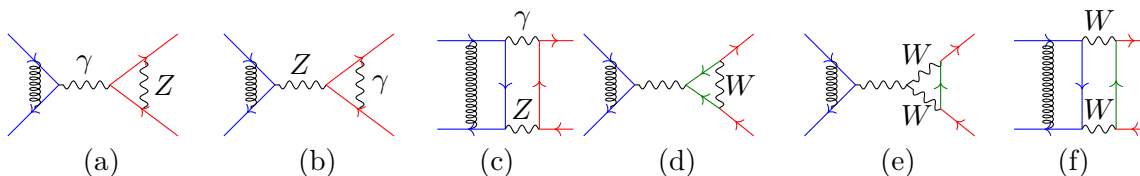
Figure 3. Sample Feynman diagrams contributing to the \gamma Z and to the WW subsets.
