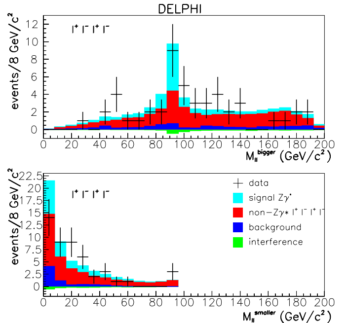
Fig. 10. Four-lepton channel: Fitted masses of two selected lepton pairs: bigger mass ( top plot ), smaller mass ( bottom plot ), compared with Standard Model predictions. The points are the data, summed over all energy points, and the histograms represent the predicted contributions to the selected event sample. In the legend, “background” means the contribution from non- l^+l^-l'^+l'^- final states
