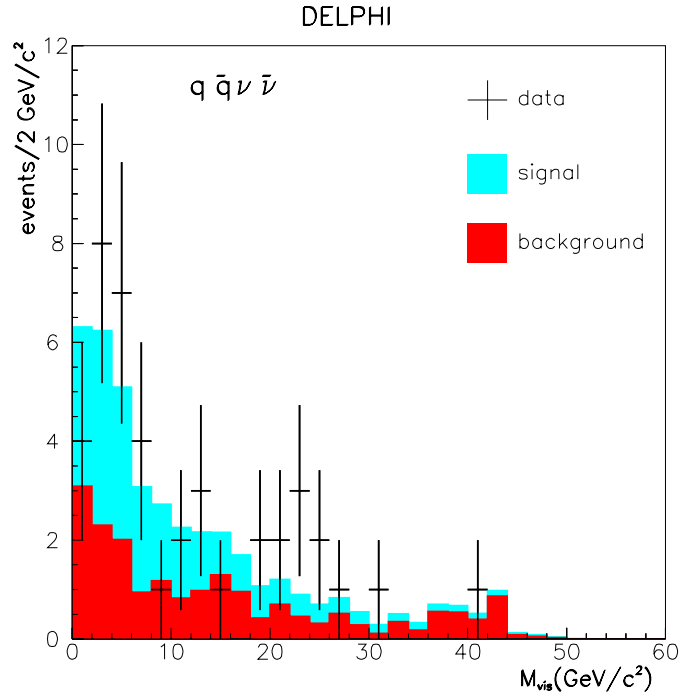
Fig. 8. Distribution of the visible invariant mass of the hadronic system in the q\bar{q}\nu\bar{\nu} selection, compared with the Standard Model predictions for signal and background. The points are the data, summed over all energy points, the light (light blue) histogram shows the predicted signal contribution, and the dark (red) histogram shows the predicted background
