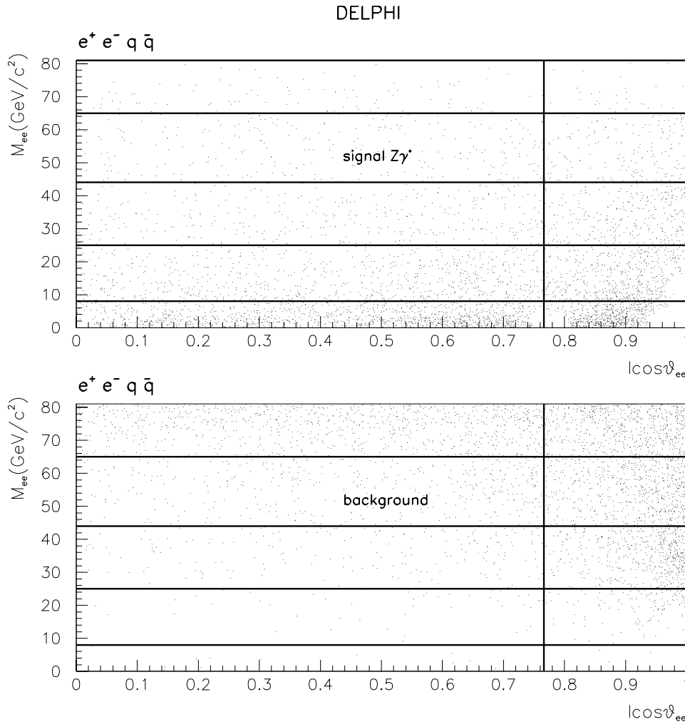
Fig. 5. Distributions of the mass of the electron-positron pair in e^+e^-q\bar{q} events for values of M_{ee} less than 80 \text{ GeV}/c^2 versus the polar direction of the pair for signal Z\gamma^* (upper plot) and background (lower plot) when the mass of the hadronic system is compatible with the Z mass. The plot shows the predictions of the Standard Model, averaged over all energy points. The binning adopted for these events follows that in Fig. 4 with an additional division into barrel and endcap regions, described in detail in the text
