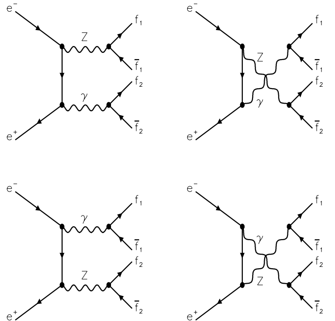
Fig. 2. Neutral current conversion diagrams for the Z\gamma^* process
