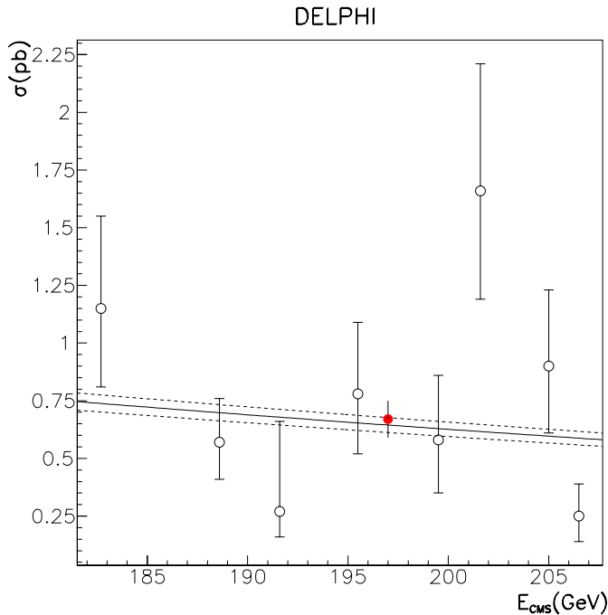
Fig. 13. Combined Z\gamma^* cross-section as a function of the centre-of-mass energy, using the matrix element signal definition (see Sect. 2). The solid line is the Standard Model prediction; the dashed line represents a 5% uncertainty around this prediction. The full (red) point is the average cross-section result, plotted at the luminosity-weighted average centre-of-mass energy
