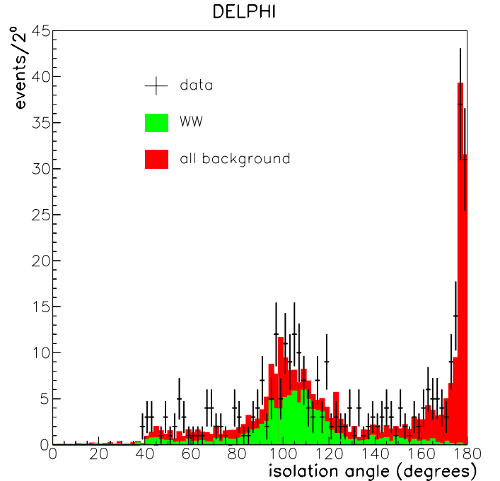
Fig. 9. Isolation angle of selected electrons, muons and single charged-particle tracks in the sample selected to mimic the background to the selected q\bar{q}\nu\bar{\nu} sample. The points are the data, summed over all energy points, the light (green) histogram is the predicted WW contribution, and the dark (red) histogram is the rest of the background
