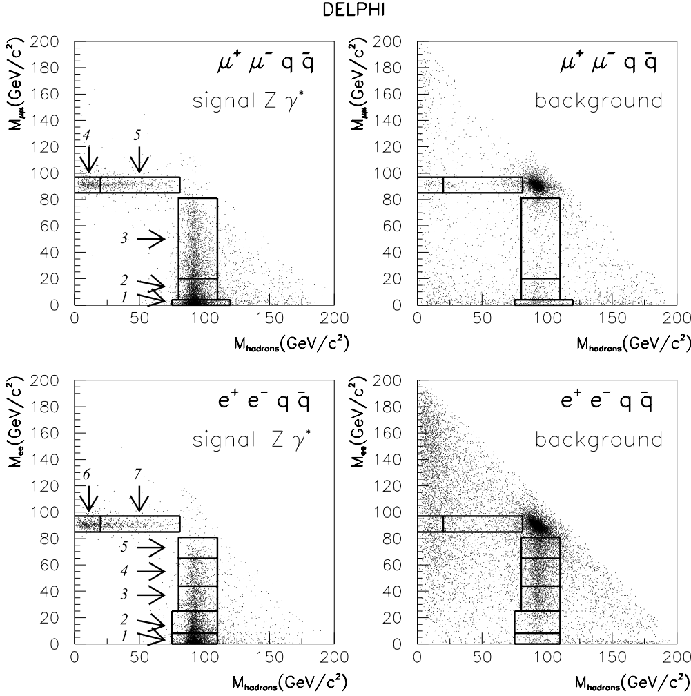
Fig. 4. l^+l^-q\bar{q} final state: Bidiimensional distributions in the plane of the di-fermion masses predicted by the Standard Model for signal Z\gamma^* (left-hand plots) and background (right-hand plots) for the two channels studied, averaged over all energy points. The bins used for the fit are also shown
