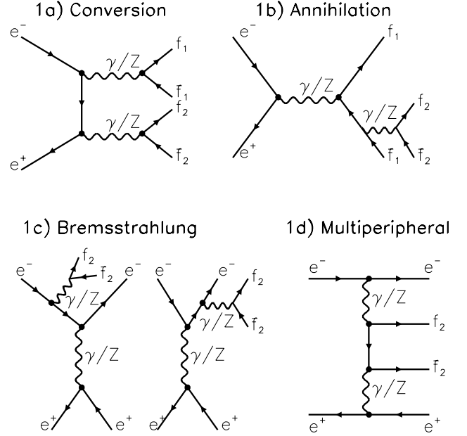
Fig. 1. The Feynman diagrams for four-fermion neutral current production in e^+e^- collisions
