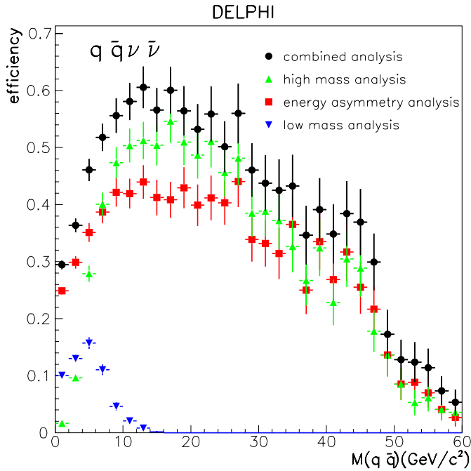
Fig. 7. Selection efficiency of the q\bar{q}\nu\bar{\nu} analyses, averaged over all energy points, as a function of the generated M(q\bar{q}) mass. The efficiency is shown for each of the three analyses (see text) separately, and for the combined analysis
