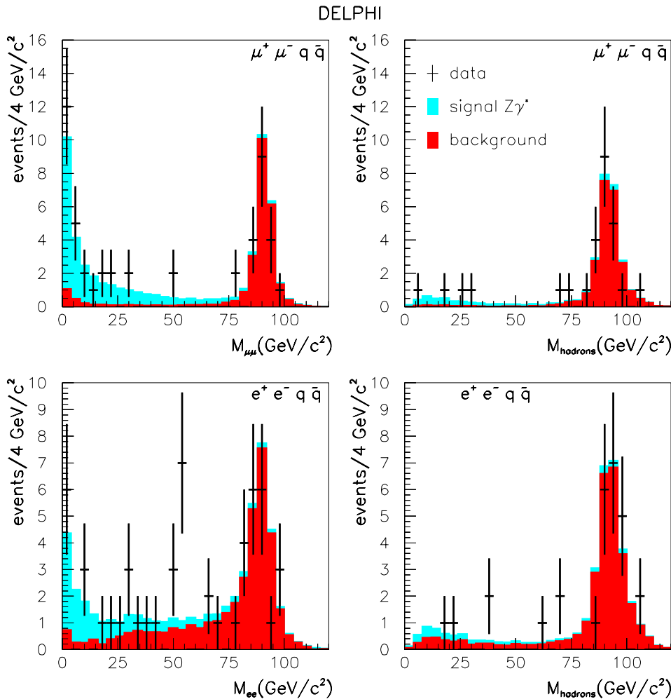
Fig. 3. l^+l^-q\bar{q} final state: Distributions of the mass of one fermion pair when the mass of the second is within 15 \text{ GeV}/c^2 of M_Z . The two lower plots are for the e^+e^-q\bar{q} channel and the two upper plots for the \mu^+\mu^-q\bar{q} channel. The points are the data summed over all energy points, the dark (red) histogram is the distribution of the background predicted by the Standard Model, and the light (light blue) histogram is the predicted distribution of the Z\gamma^* signal
