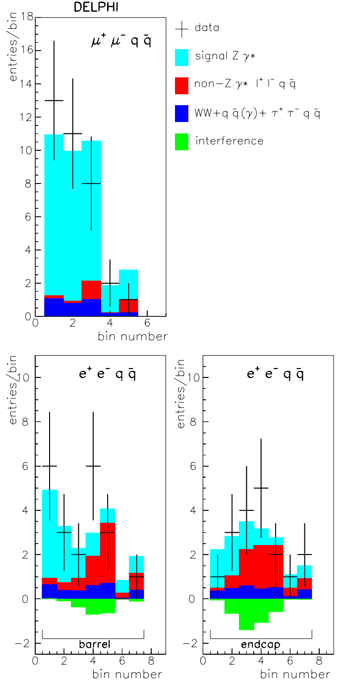
Fig. 6. Results for \mu^+\mu^-q\bar{q} (upper plot) and e^+e^-q\bar{q} (lower plots). The points are data, summed over all energy points; the shaded histograms show the results of fits to the Z\gamma^* component and the predicted Standard Model contributions from other sources. See Figs. 4 and 5 and the main text for the bin definitions
