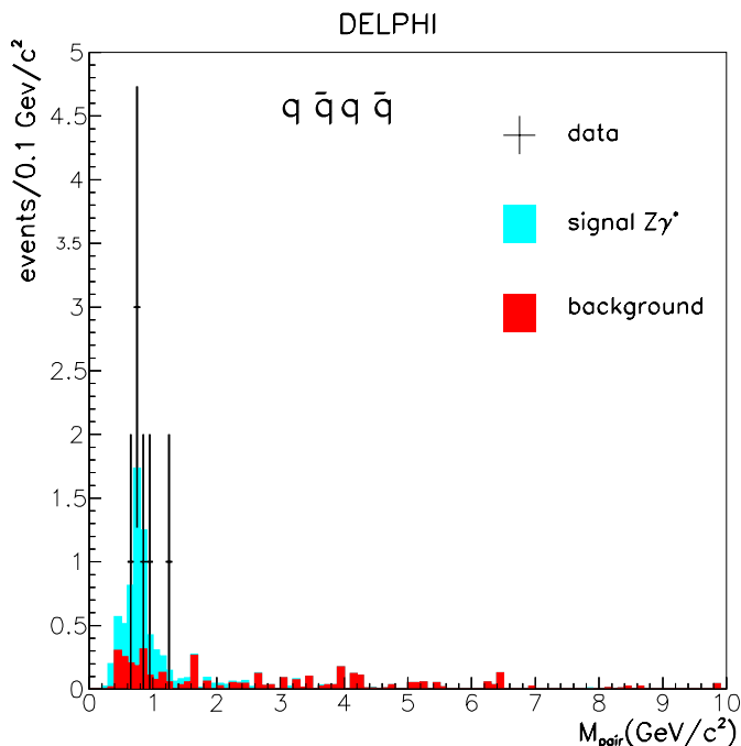
Fig. 11. The distribution of the reconstructed invariant mass of the selected pair of charged-particle tracks in the q\bar{q}q\bar{q} analysis, compared with the predictions of the Standard Model. The points are the data, summed over all energy points and shown before the final selection of M_{\text{pair}} < 2.1 \text{GeV}/c^2 ; the light (blue) histogram shows the predicted Z\gamma^* contribution, and the dark (red) histogram shows the predicted background
