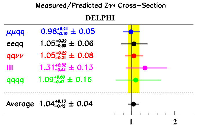
Fig. 12. Ratios of measured to predicted cross-sections for individual channels contributing to the Z\gamma^* process, using the matrix element signal definition (see Sect. 2). The vertical band displays the total error on the combination of the channels
