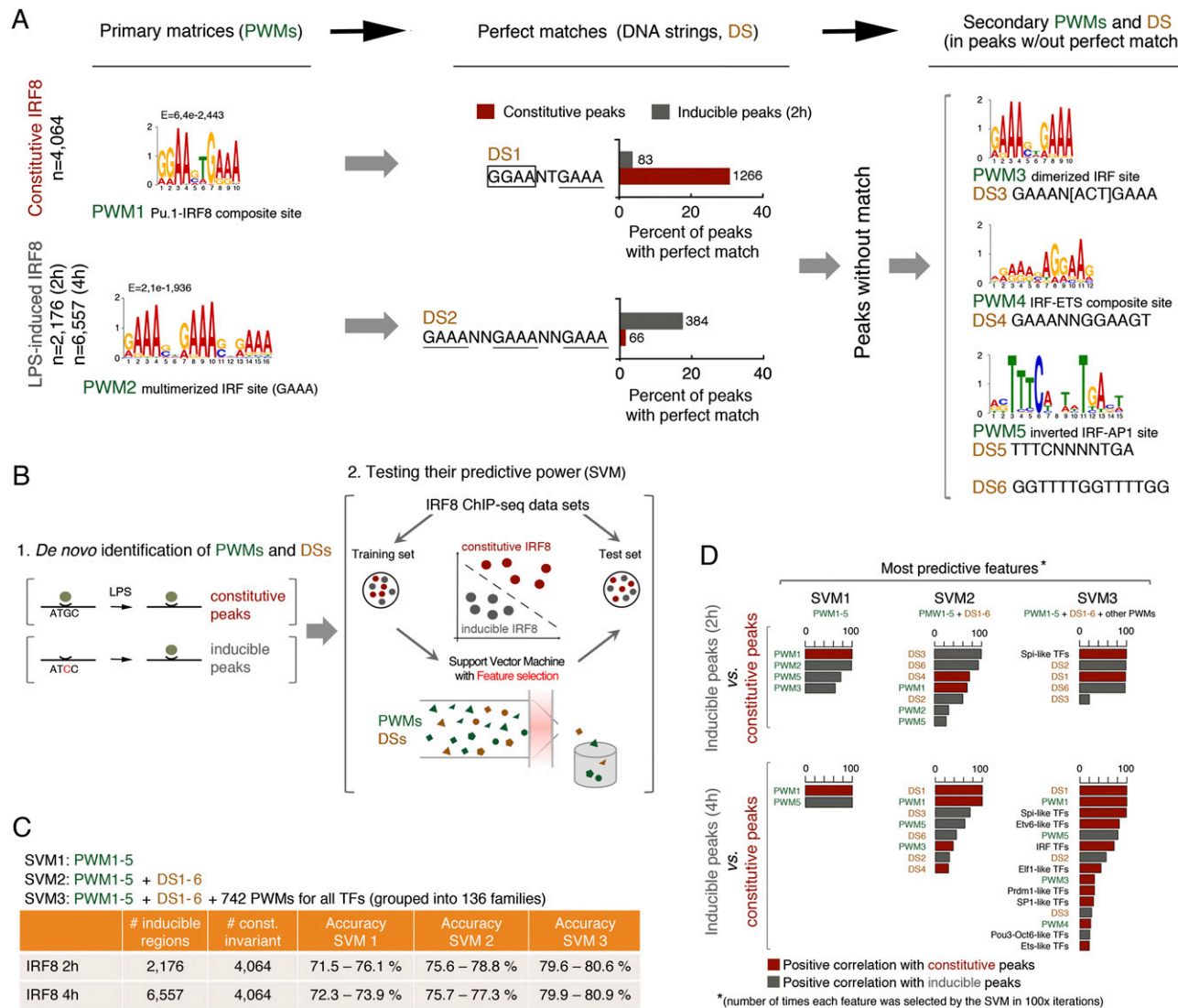
Figure 3. A small number of IRF-like DNA-binding sites predict constitutive versus LPS-inducible IRF8 recruitment. (A) Outline of the computational procedure used to retrieve sites bound by IRF8 in a constitutive or LPS-inducible manner. A de novo motif discovery approach (MEME) first retrieved PWM1 and PWM2, which were converted into DSs (DS1 and DS2, respectively) to determine the fraction of peaks in the two groups with a perfect match. Reiteration of the de novo motif discovery on the peaks without match retrieved PWM3–5 and the corresponding DSs. (B) Scheme of the SVM with feature selection used in this study. (C) The SVM was run using a combination of three sets of DNA-binding sites of increasing complexity: only PWM1–5 (SVM1), PWM1–5 and DS1–6 (SVM2), and finally, PWM1–5+DS1–6 and a set of 742 PWMs corresponding to annotated high-quality TF DNA-binding specificities (SVM3). (D) The most predictive DNA-binding sites (namely, those most frequently retrieved in 100 iterations of the three SVMs) and their association with either constitutive or LPS-inducible IRF8 peaks are shown.
