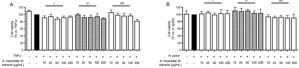
Figure S1. Cell viability (MTT test). GES-1 cells were treated for 6 h with TNF \alpha (10 ng/mL) (panel A) or H. pylori (ratio 50:1, bacteria:cell) (panel B). Results were expressed as mean \pm SEM (at least three experiments) of the relative % in comparison to stimulus (black bar), to which the value of 100% was arbitrarily assigned. I, A. erba-rotta subsp. moschata infuse; D, A. erba-rotta subsp. moschata decoction; HE, A. erba-rotta subsp. moschata hydroethanolic extract.
