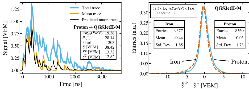
Figure 12. Left: example of a predicted trace for a simulation of a proton generated air shower done with QGSJetII-04. Right: distribution of \widehat{S}^\mu - S^\mu for all the stations in the bin specified for simulations using proton and iron nuclei.
