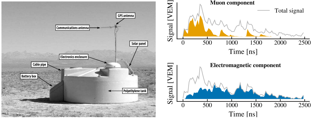
Figure 1. Left: a schematic view of a surface detector station in the field, showing its main components. Right: signal in time measured by a single station of the SD for a simulated event. The total signal corresponds to the signal that can be measured by the SD. The signal from the electromagnetic and muon components are shown independently, as this information is available in simulations. The total signal is the sum of the muon component and the electromagnetic component. Our goal is to obtain the muon component using the total signal as an input.
